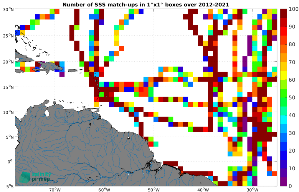
Figure 5: Number of SSS match-ups between TSG (GOSUD-Sailing-ship) SSS and the SMOS SSS L3 v2 - 9-Days (BEC) SSS product for the Amazon and Orinoco river plumes Pi-MEP region over 1^\circ \times 1^\circ boxes and for the full satellite product period.
