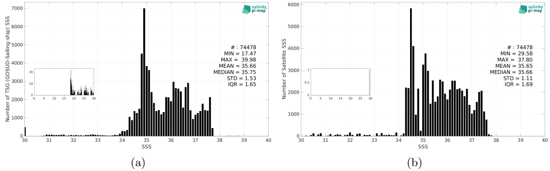
Figure 3: Histograms of SSS from TSG (GOSUD-Sailing-ship) (a) and SMOS SSS L3 v2 - 9-Days (BEC) (b) considering all match-up pairs per bins of 0.1 over the Amazon and Orinoco river plumes Pi-MEP region and for the full satellite product period.
