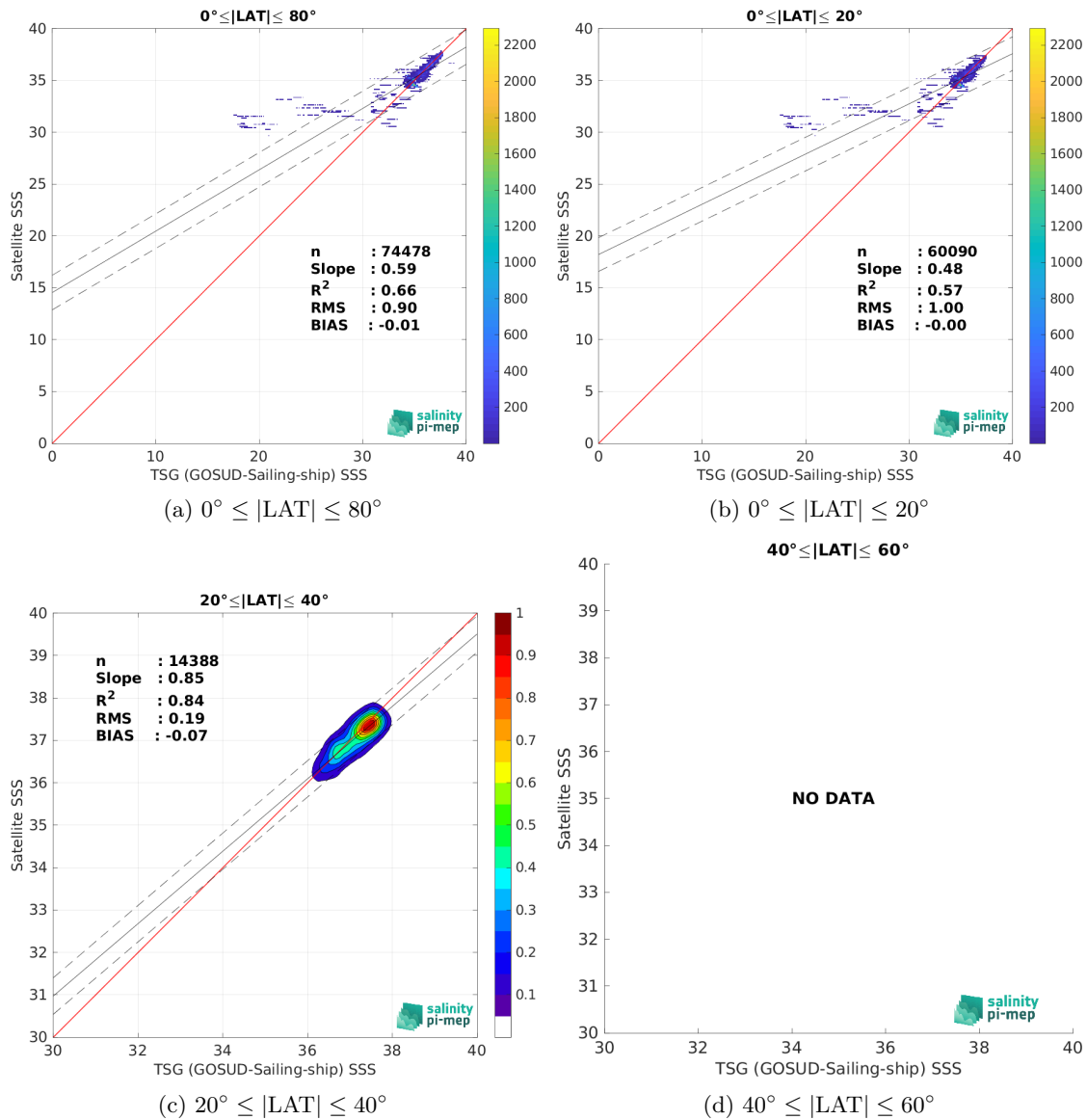
Figure 10: Contour maps of the concentration of SMOS SSS L3 v2 - 9-Days (BEC) SSS (y-axis) versus TSG (GOSUD-Sailing-ship) SSS (x-axis) at match-up pairs for different latitude bands. For each plot, the red line shows x=y . The black thin and dashed lines indicate a linear fit through the data cloud and the \pm 95\% confidence levels, respectively. The number match-up pairs n , the slope and R^2 coefficient of the linear fit, the root mean square (RMS) and the mean bias between satellite and in situ data are indicated for each latitude band in each plots.
