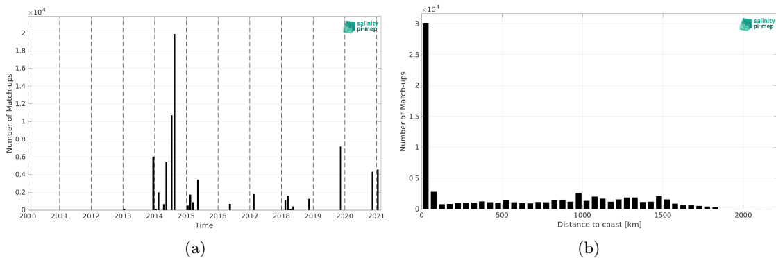
Figure 2: Number of match-ups between TSG (GOSUD-Sailing-ship) and SMOS SSS L3 v2 - 9-Days (BEC) SSS as a function of time (a) and as function of the distance to coast (b) over the Amazon and Orinoco river plumes Pi-MEP region and for the full satellite product period.
