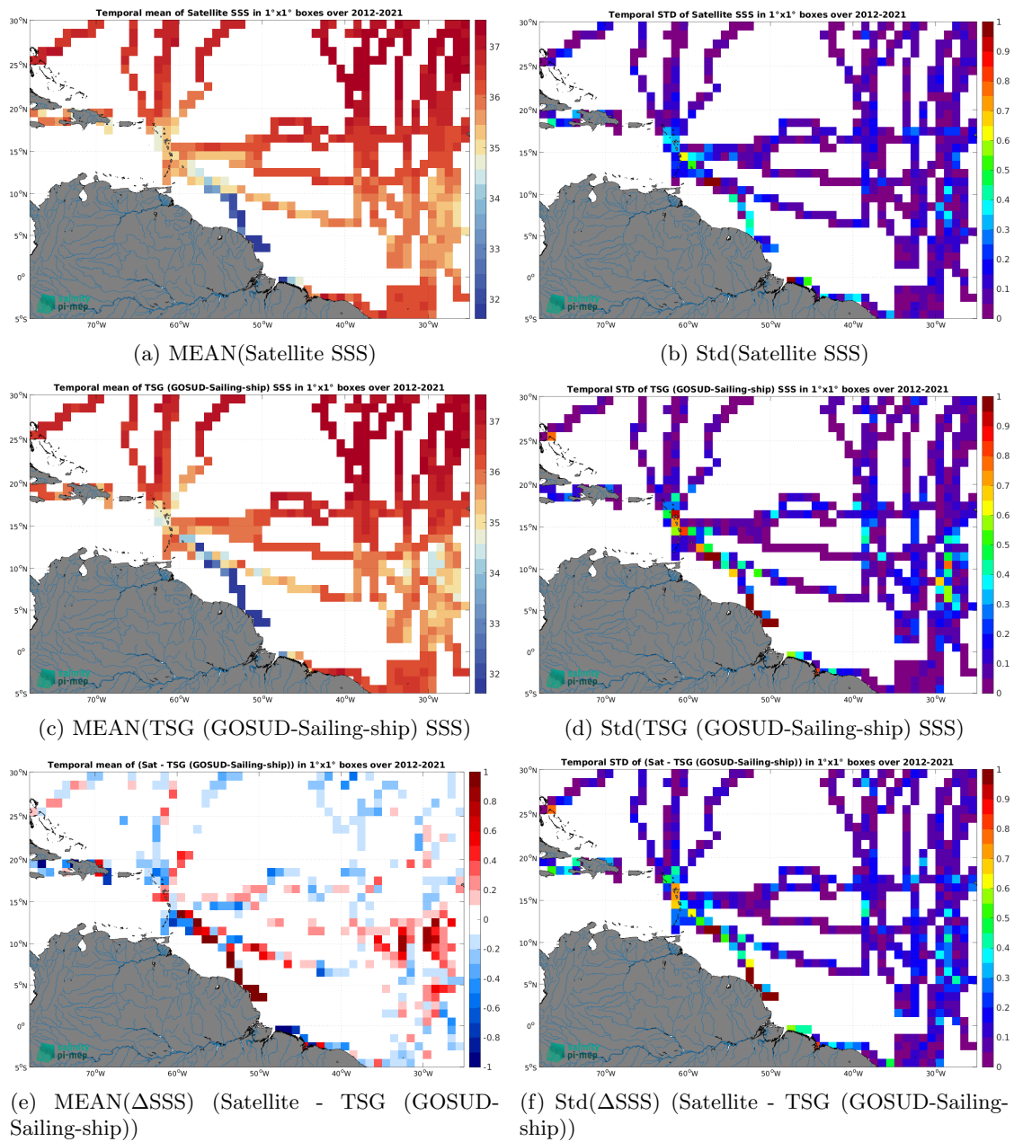
Figure 7: Temporal mean (left) and Std (right) of SSS from SMOS SSS L3 v2 - 9-Days (BEC) (top), TSG (GOSUD-Sailing-ship) (middle), and of \Delta SSS (Satellite - TSG (GOSUD-Sailing-ship)). Only match-up pairs are used to generate these maps.
