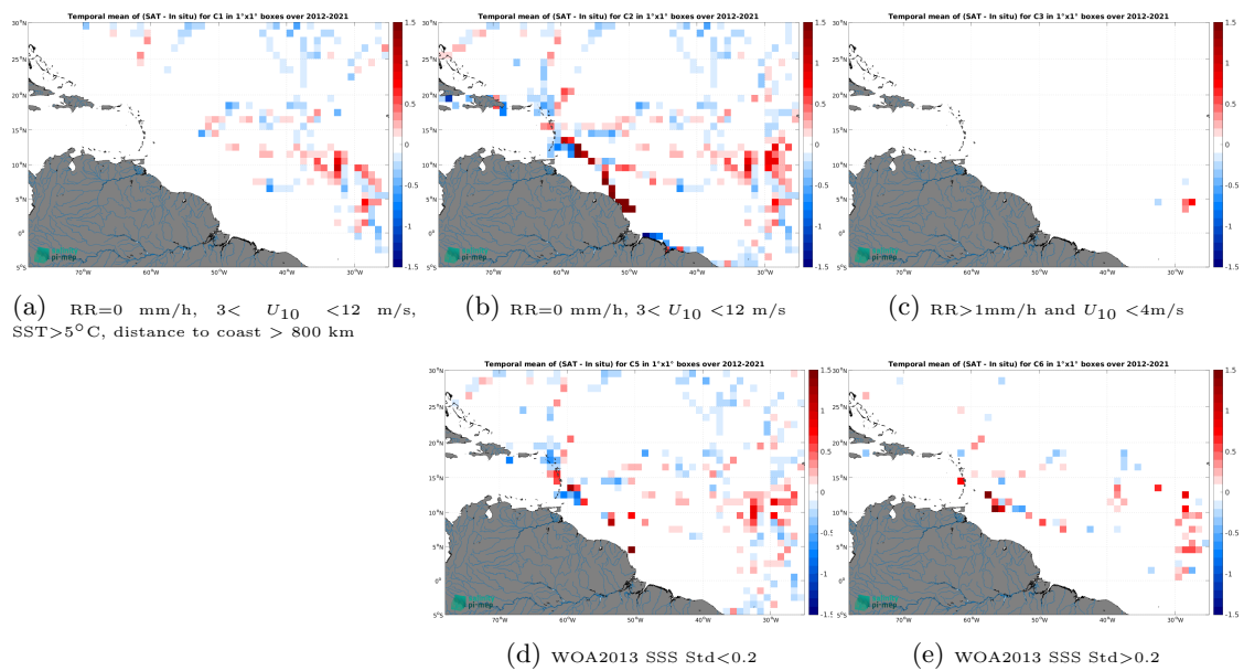
Figure 14: Temporal mean gridded over spatial boxes of size 1^\circ \times 1^\circ of \Delta SSS (SMOS SSS L3 v2 - 9-Days (BEC) - TSG (GOSUD-Sailing-ship)) for 5 different subdatasets corresponding to:RR=0 mm/h, 3 < U_{10} < 12 m/s, SST >5^\circ C, distance to coast > 800 km (a), RR=0 mm/h, 3 < U_{10} < 12 m/s (b), RR >1 mm/h and U_{10} < 4 m/s (c), WOA2013 SSS Std <0.2 (d), WOA2013 SSS Std >0.2 (e).
