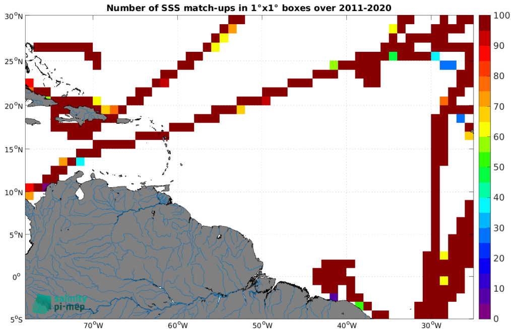
Figure 5: Number of SSS match-ups between TSG (CSIC-UTM) SSS and the SMOS SSS L3 v2 - 9-Days (BEC) SSS product for the Amazon and Orinoco river plumes Pi-MEP region over 1^\circ \times 1^\circ boxes and for the full satellite product period.
