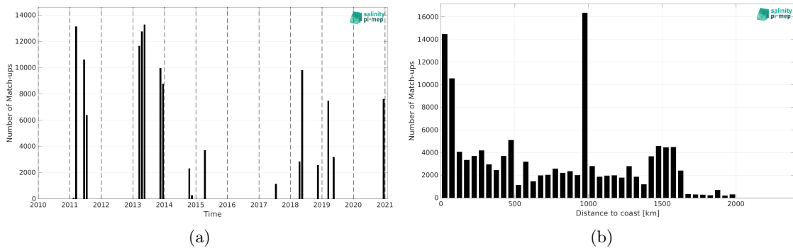
Figure 2: Number of match-ups between TSG (CSIC-UTM) and SMOS SSS L3 v2 - 9-Days (BEC) SSS as a function of time (a) and as function of the distance to coast (b) over the Amazon and Orinoco river plumes Pi-MEP region and for the full satellite product period.
