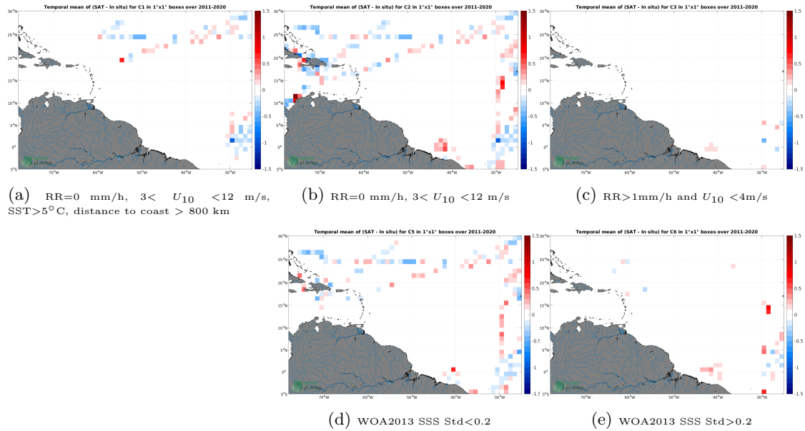
Figure 12: Temporal mean gridded over spatial boxes of size 1^\circ \times 1^\circ of \Delta SSS (SMOS SSS L3 v2 - 9-Days (BEC) - TSG (CSIC-UTM)) for 5 different subdatasets corresponding to:RR=0 mm/h, 3 < U_{10} < 12 m/s, SST >5^\circ\text{C} , distance to coast > 800 km (a), RR=0 mm/h, 3 < U_{10} < 12 m/s (b), RR >1 mm/h and U_{10} < 4 m/s (c), WOA2013 SSS Std <0.2 (d), WOA2013 SSS Std >0.2 (e).
