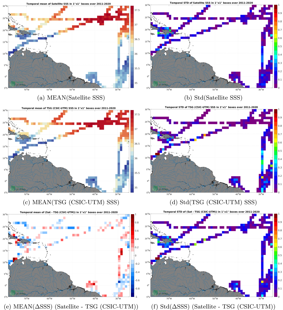
Figure 6: Temporal mean (left) and Std (right) of SSS from SMOS SSS L3 v2 - 9-Days (BEC) (top), TSG (CSIC-UTM) (middle), and of \Delta SSS (Satellite - TSG (CSIC-UTM)). Only match-up pairs are used to generate these maps.
