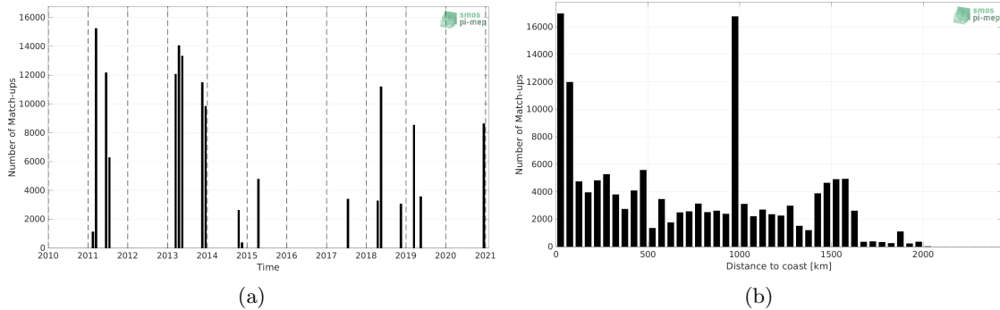
Figure 1: Number of match-ups between TSG (CSIC-UTM) and SMOS SSS L3 v2 - 9-Days (BEC) SSS as a function of time (a) and as function of the distance to coast (b) over the Amazon and Orinoco river plumes Pi-MEP region and for the full satellite product period.
