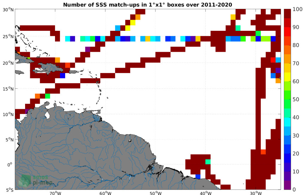
Figure 4: Number of SSS match-ups between TSG (CSIC-UTM) SSS and the SMOS SSS L3 v2 - 9-Days (BEC) SSS product for the Amazon and Orinoco river plumes Pi-MEP region over 1^{\circ} \times 1^{\circ} boxes and for the full satellite product period.
