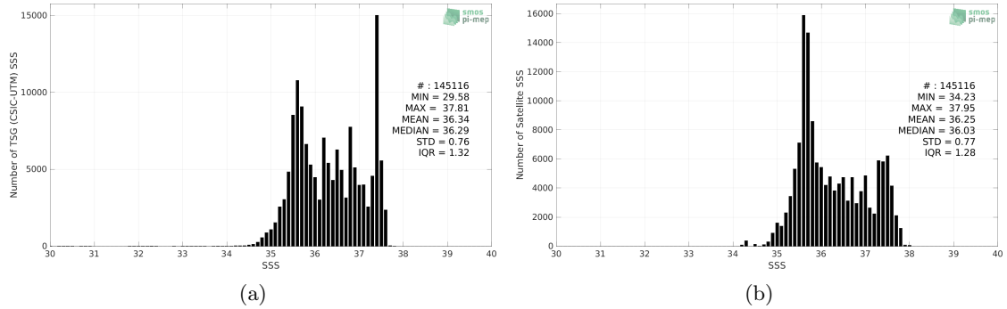
Figure 2: Histograms of SSS from TSG (CSIC-UTM) (a) and SMOS SSS L3 v2 - 9-Days (BEC) (b) considering all match-up pairs per bins of 0.1 over the Amazon and Orinoco river plumes Pi-MEP region and for the full satellite product period.
