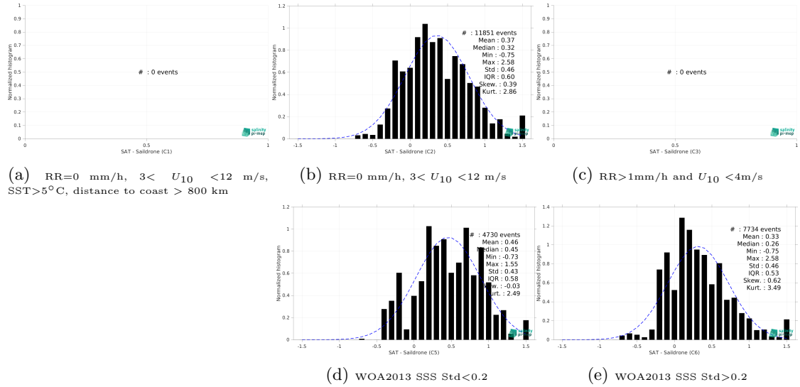
Figure 15: Normalized histogram of \Delta SSS (SMOS SSS L3 v2 - 9-Days (BEC) - Saildrone) for 5 different subdatasets corresponding to: RR=0 mm/h, 3 < U_{10} < 12 m/s, SST>5°C, distance to coast > 800 km (a), RR=0 mm/h, 3 < U_{10} < 12 m/s (b), RR>1mm/h and U_{10} < 4 m/s (c), WOA2013 SSS Std<0.2 (d), WOA2013 SSS Std>0.2 (e).
