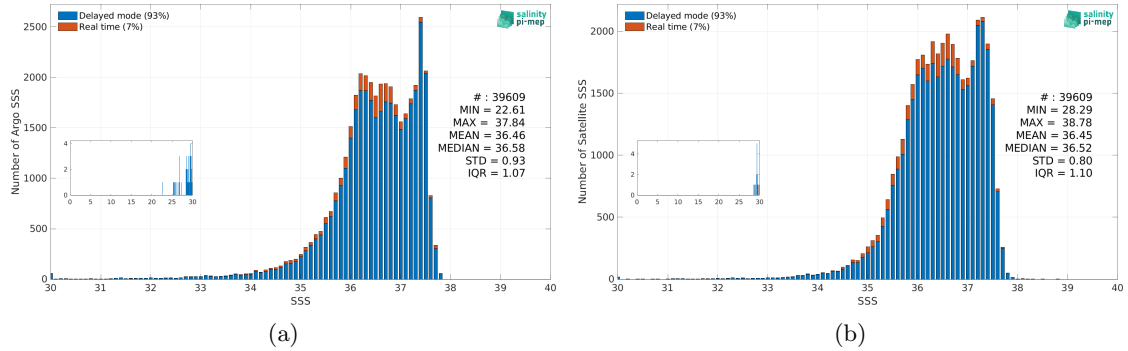
Figure 3: Histograms of SSS from Argo (a) and SMOS SSS L3 v2 - 9-Days (BEC) (b) considering all match-up pairs per bins of 0.1 over the Amazon and Orinoco river plumes Pi-MEP region and for the full satellite product period.
