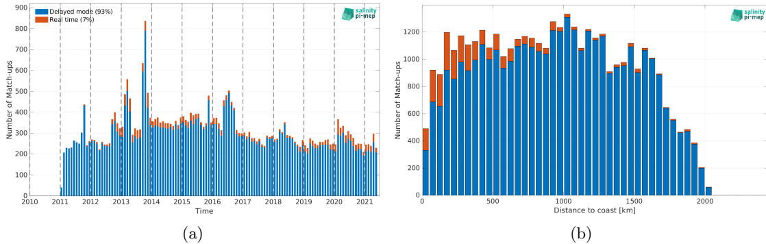
Figure 2: Number of match-ups between Argo and SMOS SSS L3 v2 - 9-Days (BEC) SSS as a function of time (a) and as function of the distance to coast (b) over the Amazon and Orinoco river plumes Pi-MEP region and for the full satellite product period.
