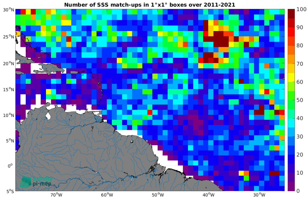
Figure 5: Number of SSS match-ups between Argo SSS and the SMOS SSS L3 v2 - 9-Days (BEC) SSS product for the Amazon and Orinoco river plumes Pi-MEP region over 1^{\circ} \times 1^{\circ} boxes and for the full satellite product period.
