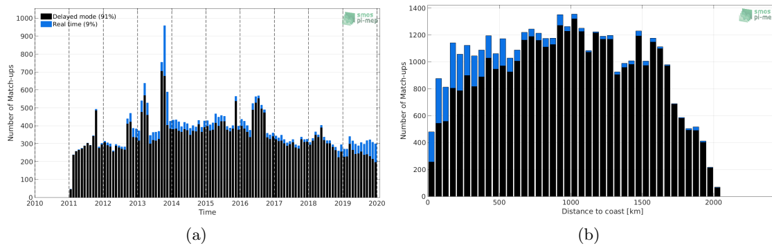
Figure 1: Number of match-ups between Argo and SMOS SSS L3 v2 - 9-Days (BEC) SSS as a function of time (a) and as function of the distance to coast (b) over the Amazon and Orinoco river plumes Pi-MEP region and for the full satellite product period.
