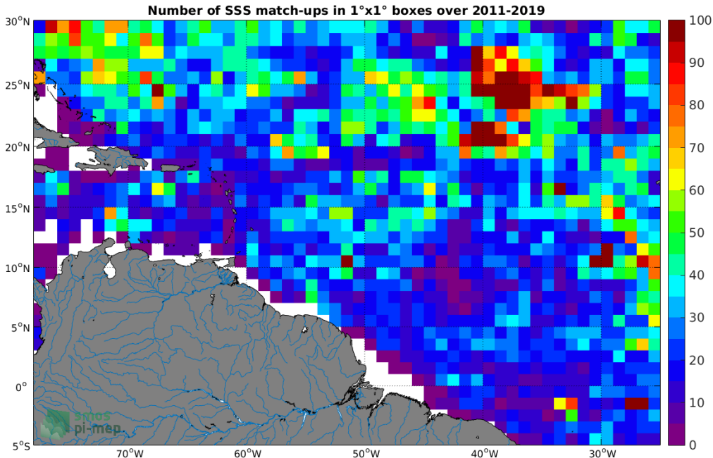
Figure 4: Number of SSS match-ups between Argo SSS and the SMOS SSS L3 v2 - 9-Days (BEC) SSS product for the Amazon and Orinoco river plumes Pi-MEP region over 1^{\circ} \times 1^{\circ} boxes and for the full satellite product period.
