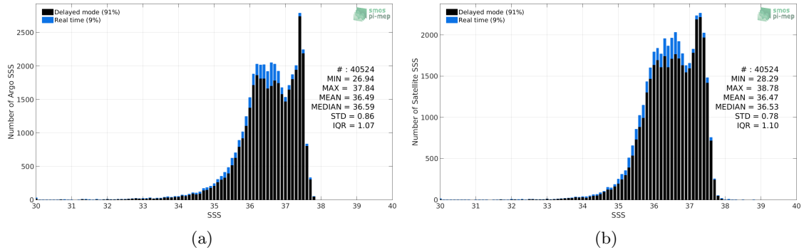
Figure 2: Histograms of SSS from Argo (a) and SMOS SSS L3 v2 - 9-Days (BEC) (b) considering all match-up pairs per bins of 0.1 over the Amazon and Orinoco river plumes Pi-MEP region and for the full satellite product period.
