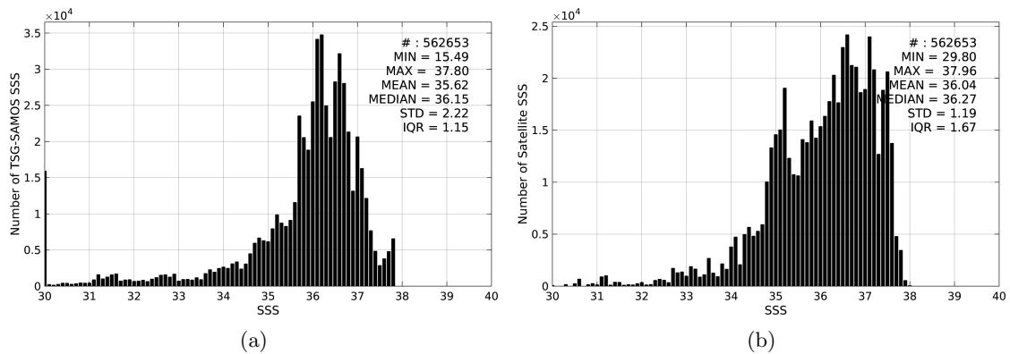
Figure 2: Histograms of SSS from TSG-SAMOS (a) and SMOS-L3-BEC-OA-V1-9DAYS-0.25DEG (b) considering all match-up pairs per bins of 0.1 over the Amazon and Orinoco river plumes Pi-MEP region and for the full satellite product period.
