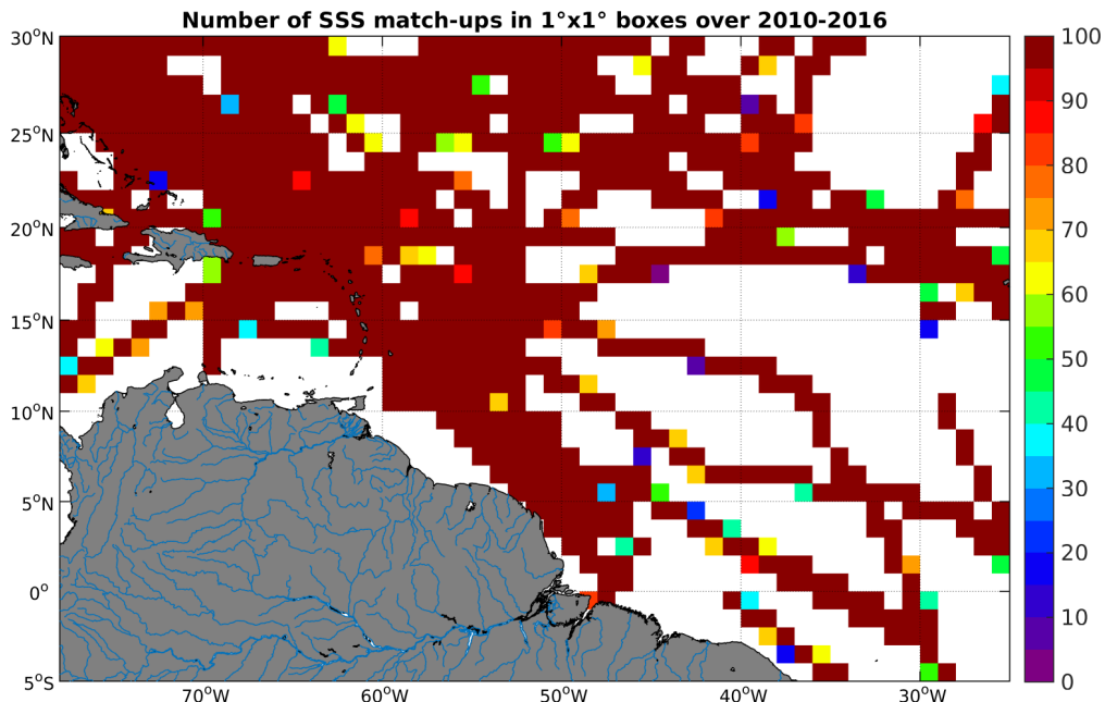
Figure 4: Number of SSS match-ups between TSG-SAMOS SSS and the SMOS-L3-BEC-OA-V1-9DAYS-0.25DEG SSS product for the Amazon and Orinoco river plumes Pi-MEP region over 1^\circ \times 1^\circ boxes and for the full satellite product period.
