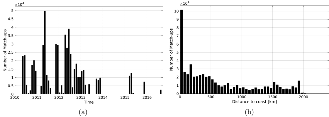
Figure 1: Number of match-ups between TSG-SAMOS and SMOS-L3-BEC-OA-V1-9DAYS-0.25DEG SSS as a function of time (a) and as function of the distance to coast (b) over the Amazon and Orinoco river plumes Pi-MEP region and for the full satellite product period.
