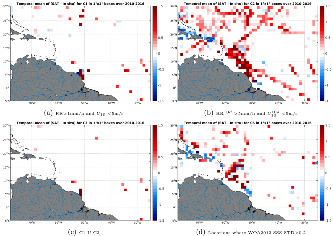
Figure 12: Temporal mean gridded over spatial boxes of size 1^\circ \times 1^\circ of \Delta SSS (SMOS-L3-BEC-OA-V1-9DAYS-0.25DEG - TSG-SAMOS) for 4 different subdatasets corresponding to: RR > 1\text{mm/h} and U_{10} < 5\text{m/s} (a), RR^{10d} > 5\text{mm/h} and U_{10}^{10d} < 5\text{m/s} (b), C1 U C2 (c), Locations where WOA2013 SSS STD > 0.2 (d).
