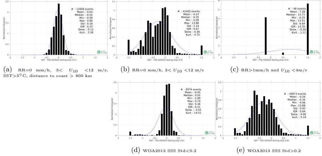
Figure 13: Normalized histogram of \Delta\text{SSS} (SMOS-L3-BEC-OA-V1-9DAYS-0.25DEG - TSG-GOSUD-Sailing-ship) for 5 different subdatasets corresponding to: RR=0 mm/h, 3 < U_{10} < 12 m/s, SST > 5^\circ\text{C} , distance to coast > 800 km (a), RR=0 mm/h, 3 < U_{10} < 12 m/s (b), RR > 1\text{mm/h} and U_{10} < 4\text{m/s} (c), WOA2013 SSS Std < 0.2 (d), WOA2013 SSS Std > 0.2 (e).
