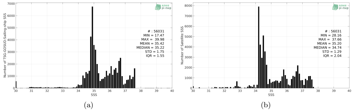
Figure 2: Histograms of SSS from TSG-GOSUD-Sailing-ship (a) and SMOS-L3-BEC-OA-V1-9DAYS-0.25DEG (b) considering all match-up pairs per bins of 0.1 over the Amazon and Orinoco river plumes Pi-MEP region and for the full satellite product period.
