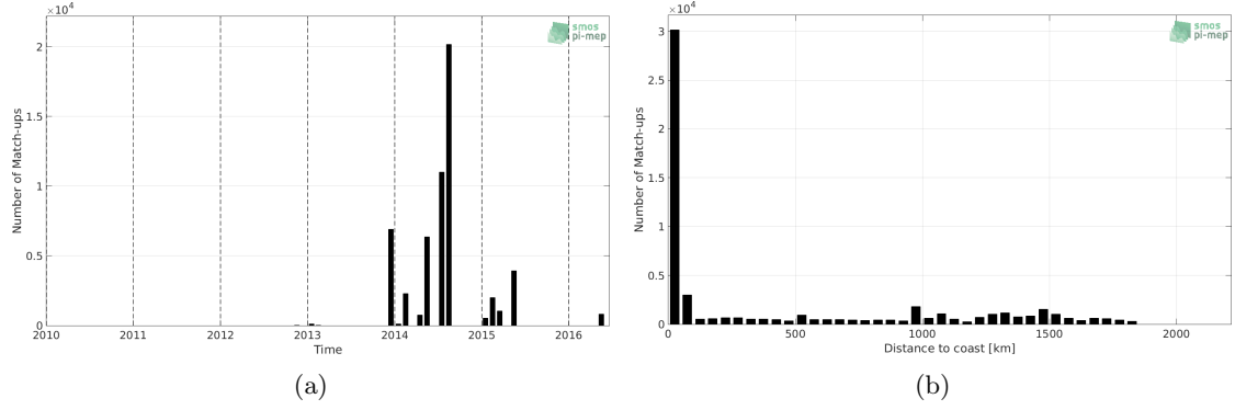
Figure 1: Number of match-ups between TSG-GOSUD-Sailing-ship and SMOS-L3-BEC-OA-V1-9DAYS-0.25DEG SSS as a function of time (a) and as function of the distance to coast (b) over the Amazon and Orinoco river plumes Pi-MEP region and for the full satellite product period.
