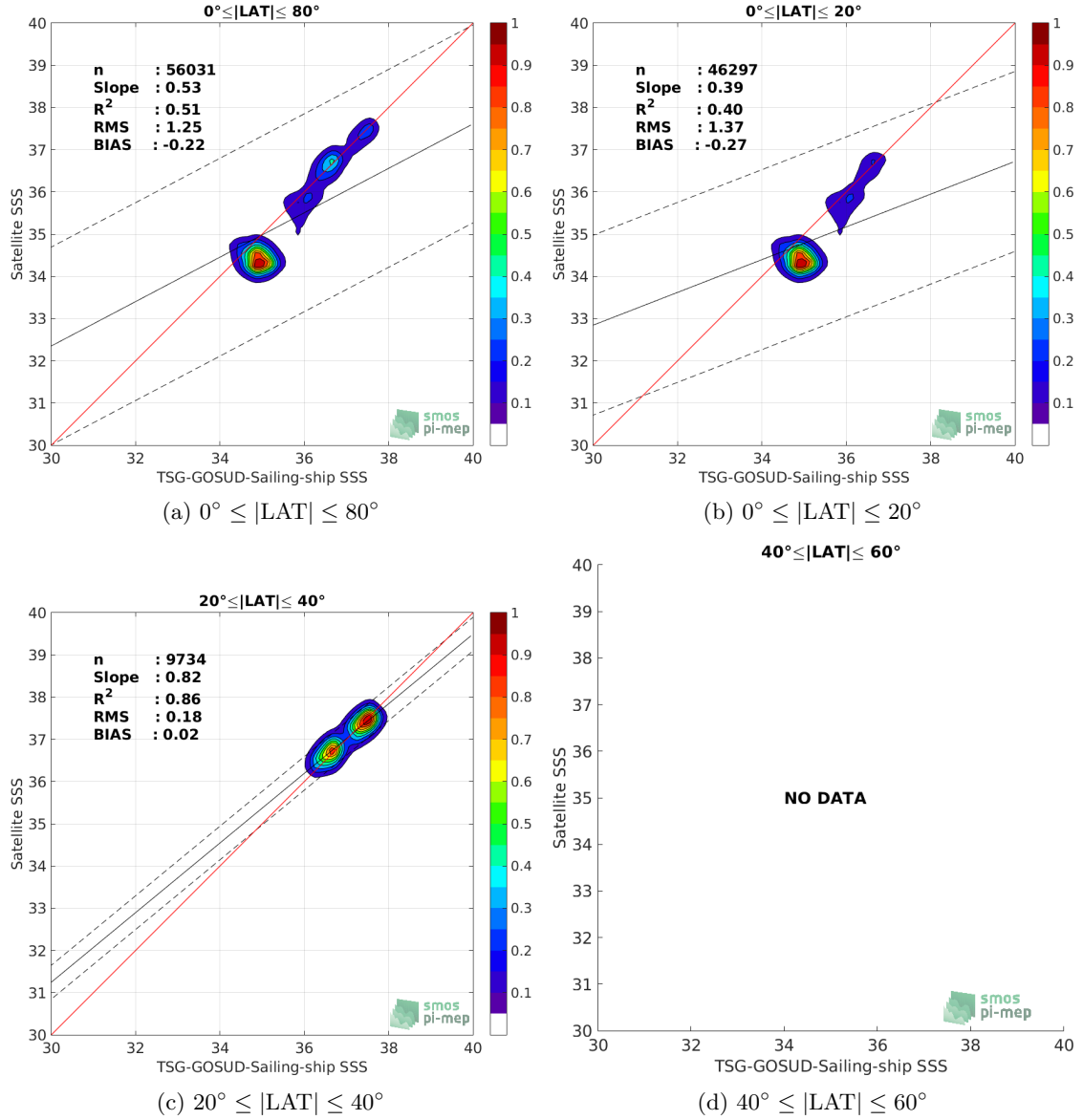
Figure 9: Contour maps of the concentration of SMOS-L3-BEC-OA-V1-9DAYS-0.25DEG SSS (y-axis) versus TSG-GOSUD-Sailing-ship SSS (x-axis) at match-up pairs for different latitude bands. For each plot, the red line shows x=y . The black thin and dashed lines indicate a linear fit through the data cloud and the \pm 95\% confidence levels, respectively. The number match-up pairs n , the slope and R^2 coefficient of the linear fit, the root mean square (RMS) and the mean bias between satellite and in situ data are indicated for each latitude band in each plot.
