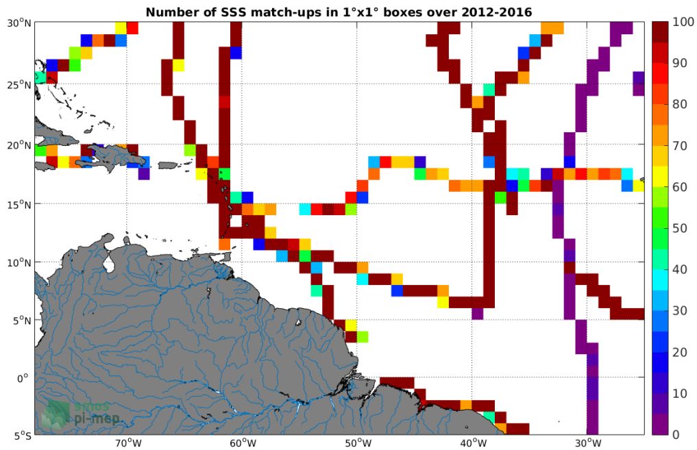
Figure 4: Number of SSS match-ups between TSG-GOSUD-Sailing-ship SSS and the SMOS-L3-BEC-OA-V1-9DAYS-0.25DEG SSS product for the Amazon and Orinoco river plumes Pi-MEP region over 1°x1° boxes and for the full satellite product period.
