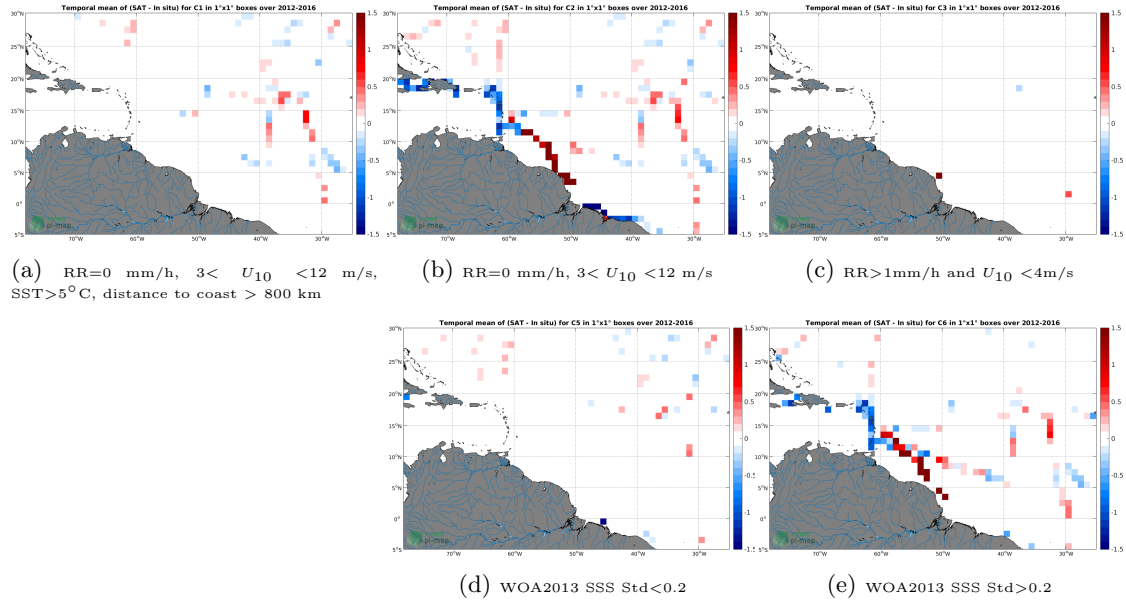
Figure 12: Temporal mean gridded over spatial boxes of size 1^\circ \times 1^\circ of \Delta SSS (SMOS-L3-BEC-OA-V1-9DAYS-0.25DEG - TSG-GOSUD-Sailing-ship) for 5 different subdatasets corresponding to: RR=0 mm/h, 3 < U_{10} < 12 m/s, SST > 5^\circ C , distance to coast > 800 km (a), RR=0 mm/h, 3 < U_{10} < 12 m/s (b), RR > 1 mm/h and U_{10} < 4 m/s (c), WOA2013 SSS Std < 0.2 (d), WOA2013 SSS Std > 0.2 (e).
