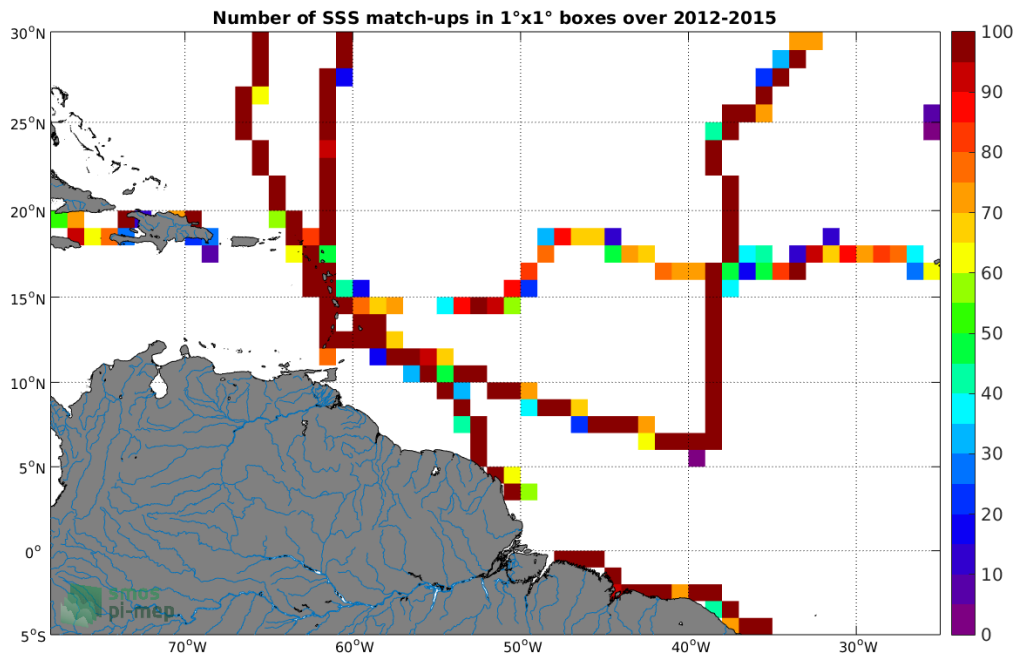
Figure 4: Number of SSS match-ups between TSG-GOSUD-Sailing-ship SSS and the SMOS-L3-BEC-OA-V1-9DAYS-0.25DEG SSS product for the Amazon and Orinoco river plumes Pi-MEP region over 1^\circ \times 1^\circ boxes and for the full satellite product period.
