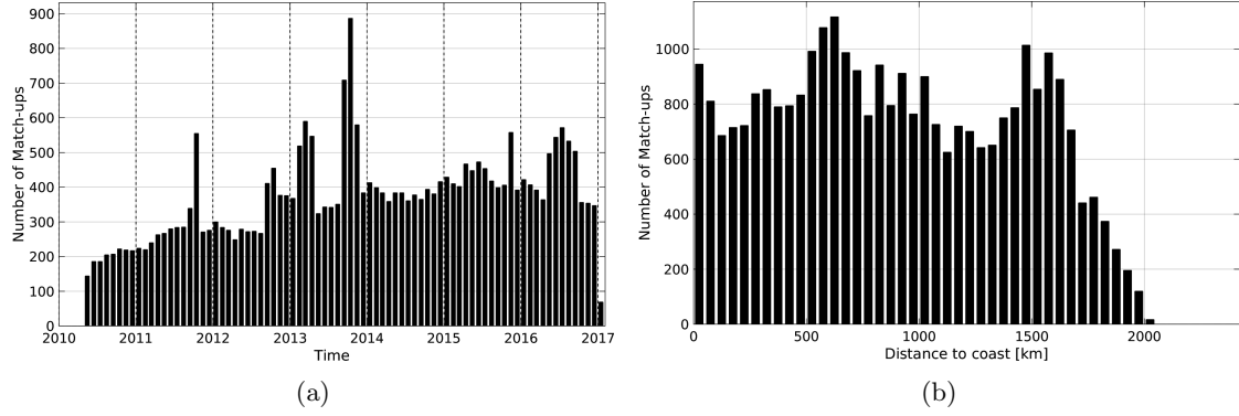
Figure 1: Number of match-ups between Argo and SMOS-L3-BEC-OA-V1-9DAYS-0.25DEG SSS as a function of time (a) and as function of the distance to coast (b) over the Amazon and Orinoco river plumes Pi-MEP region and for the full satellite product period.
