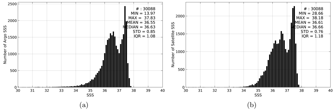
Figure 2: Histograms of SSS from Argo (a) and SMOS-L3-BEC-OA-V1-9DAYS-0.25DEG (b) considering all match-up pairs per bins of 0.1 over the Amazon and Orinoco river plumes Pi-MEP region and for the full satellite product period.
