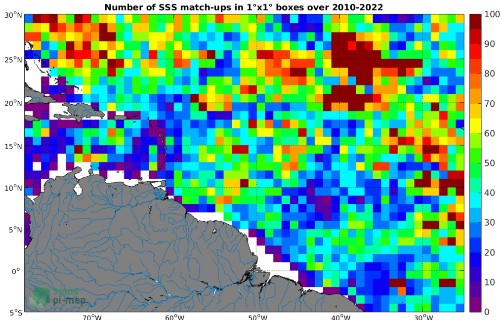
Figure 4: Number of SSS match-ups between Argo SSS and the SMOS SSS L2-AVERAGED v700 (ESA) SSS product for the Amazon and Orinoco river plumes Pi-MEP region over 1^\circ \times 1^\circ boxes and for the full satellite product period.
