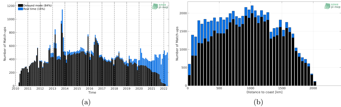
Figure 1: Number of match-ups between Argo and SMOS SSS L2-AVERAGED v700 (ESA) SSS as a function of time (a) and as function of the distance to coast (b) over the Amazon and Orinoco river plumes Pi-MEP region and for the full satellite product period.
