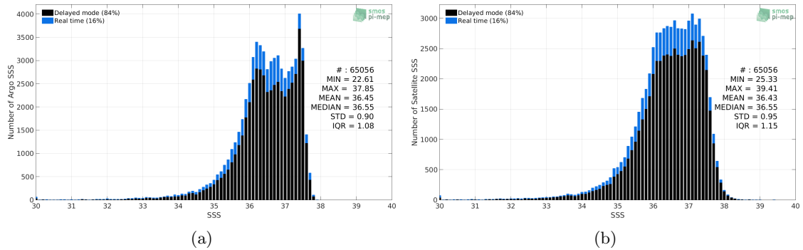
Figure 2: Histograms of SSS from Argo (a) and SMOS SSS L2-AVERAGED v700 (ESA) (b) considering all match-up pairs per bins of 0.1 over the Amazon and Orinoco river plumes Pi-MEP region and for the full satellite product period.
