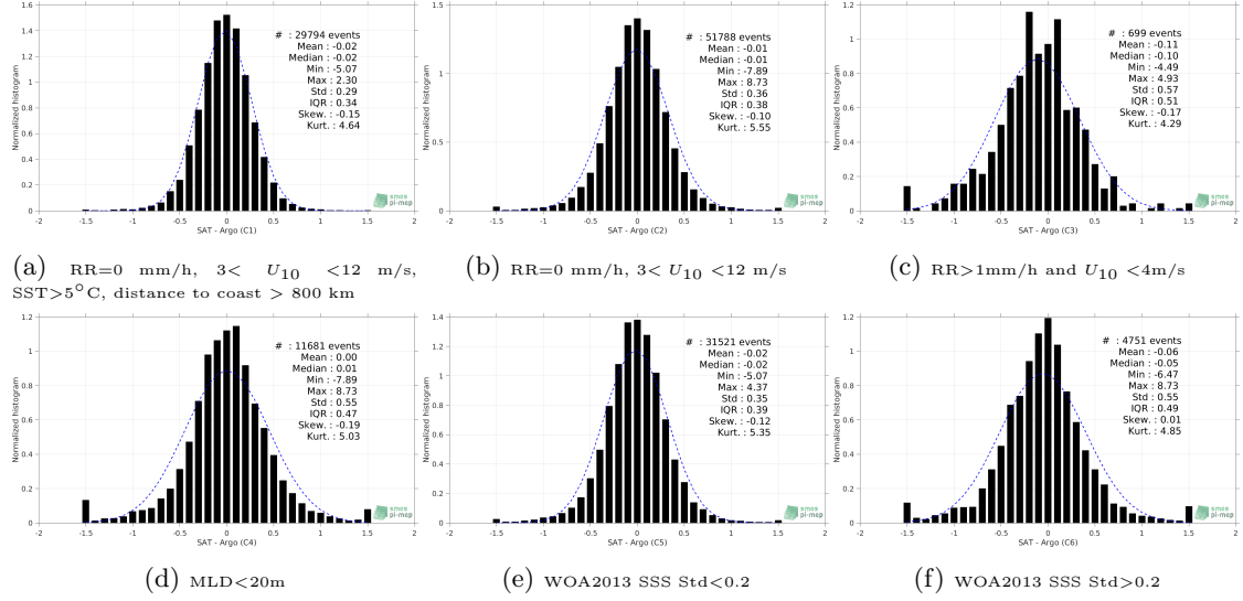
Figure 13: Normalized histogram of \Delta SSS (SMOS SSS L2-AVERAGED v700 (ESA) - Argo) for 6 different subdatasets corresponding to: RR=0 mm/h, 3 < U_{10} < 12 m/s, SST>5°C, distance to coast > 800 km (a), RR=0 mm/h, 3 < U_{10} < 12 m/s (b), RR>1mm/h and U_{10} < 4 m/s (c), MLD<20m (d), WOA2013 SSS Std<0.2 (e), WOA2013 SSS Std>0.2 (f).
