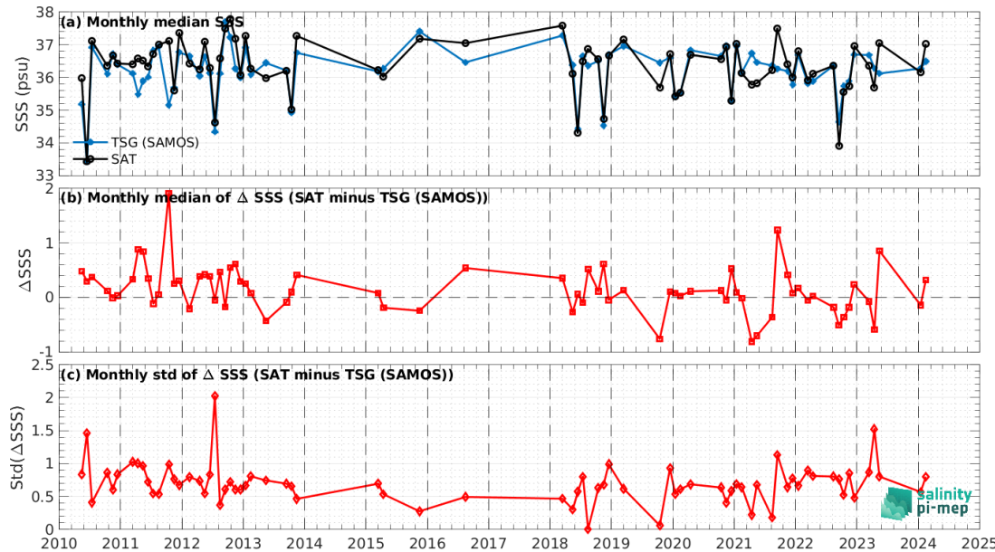
Figure 8: Time series of the monthly median SSS (top), median of \Delta\text{SSS} (Satellite - TSG (SAMOS)) and Std of \Delta\text{SSS} (Satellite - TSG (SAMOS)) over the Amazon and Orinoco river plumes Pi-MEP region considering all match-ups collected by the Pi-MEP.
