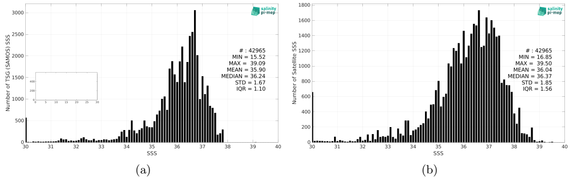
Figure 2: Histograms of SSS from TSG (SAMOS) (a) and SMOS SSS L2 v700 (ESA) (b) considering all match-up pairs per bins of 0.1 over the Amazon and Orinoco river plumes Pi-MEP region and for the full satellite product period.
