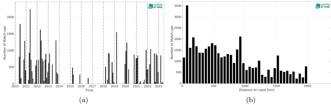
Figure 1: Number of match-ups between TSG (SAMOS) and SMOS SSS L2 v700 (ESA) SSS as a function of time (a) and as function of the distance to coast (b) over the Amazon and Orinoco river plumes Pi-MEP region and for the full satellite product period.
