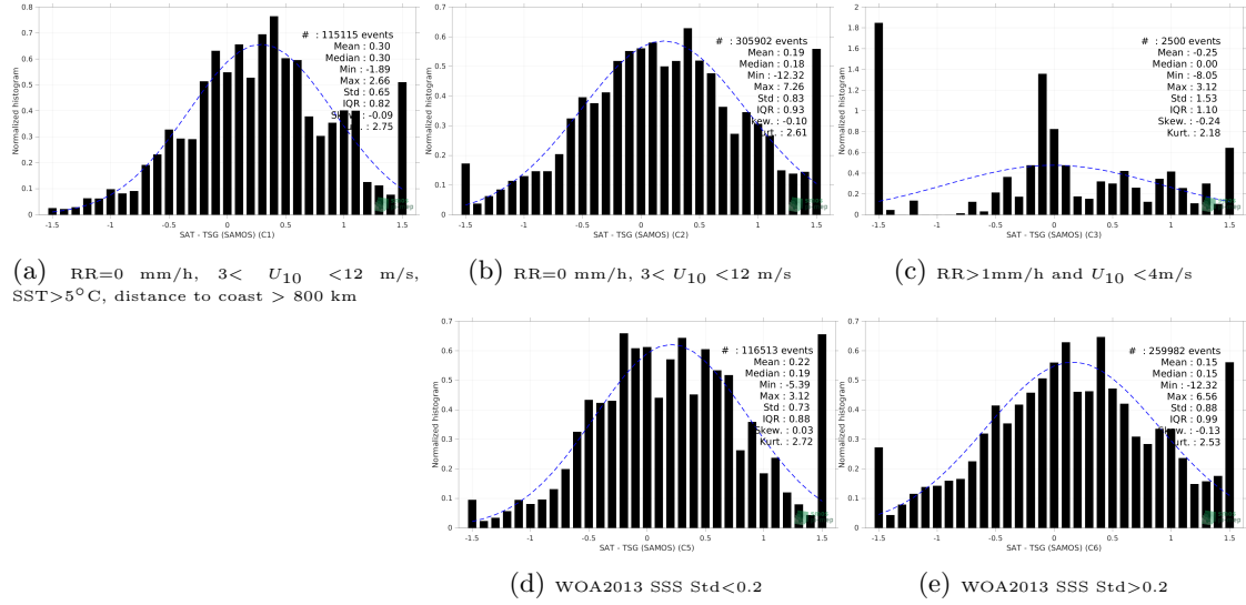
Figure 13: Normalized histogram of \Delta SSS (SMOS SSS L2 v700 (ESA) - TSG (SAMOS)) for 5 different subdatasets corresponding to: RR=0 mm/h, 3 < U_{10} < 12 m/s, SST >5^{\circ} C, distance to coast > 800 km (a), RR=0 mm/h, 3 < U_{10} < 12 m/s (b), RR >1 mm/h and U_{10} < 4 m/s (c), WOA2013 SSS Std <0.2 (d), WOA2013 SSS Std >0.2 (e).
