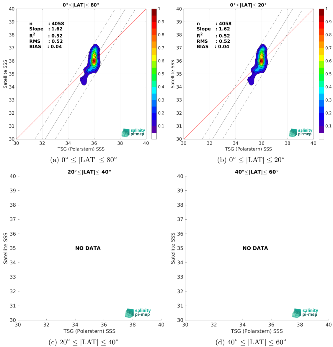
Figure 10: Contour maps of the concentration of SMOS SSS L2 v700 (ESA) SSS (y-axis) versus TSG (Polarstern) SSS (x-axis) at match-up pairs for different latitude bands. For each plot, the red line shows x=y . The black thin and dashed lines indicate a linear fit through the data cloud and the \pm 95\% confidence levels, respectively. The number match-up pairs n , the slope and R^2 coefficient of the linear fit, the root mean square (RMS) and the mean bias between satellite and in situ data are indicated for each latitude band in each plots.
