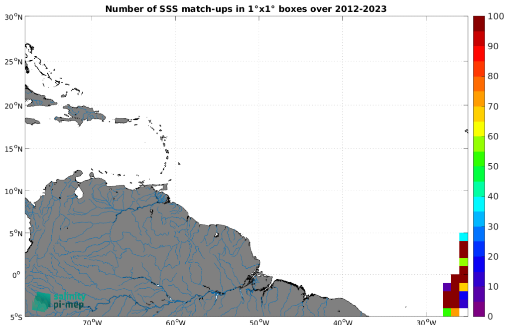
Figure 5: Number of SSS match-ups between TSG (Polarstern) SSS and the SMOS SSS L2 v700 (ESA) SSS product for the Amazon and Orinoco river plumes Pi-MEP region over 1^\circ \times 1^\circ boxes and for the full satellite product period.
