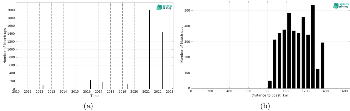
Figure 2: Number of match-ups between TSG (Polarstern) and SMOS SSS L2 v700 (ESA) SSS as a function of time (a) and as function of the distance to coast (b) over the Amazon and Orinoco river plumes Pi-MEP region and for the full satellite product period.
