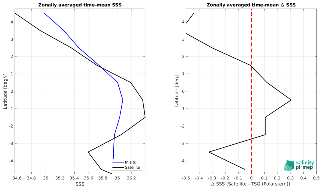
Figure 9: Left panel: Zonal mean SSS from SMOS SSS L2 v700 (ESA) satellite product (black) and from TSG (Polarstern) (blue). Right panel: Zonal mean of \Delta SSS (Satellite - TSG (Polarstern)) for all the collected Pi-MEP match-up pairs estimated over the full satellite product period.
