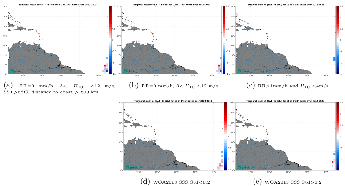
Figure 14: Temporal mean gridded over spatial boxes of size 1^\circ \times 1^\circ of \Delta SSS (SMOS SSS L2 v700 (ESA) - TSG (Polarstern)) for 5 different subdatasets corresponding to:RR=0 mm/h, 3 < U_{10} < 12 m/s, SST >5^\circ\text{C} , distance to coast > 800 km (a), RR=0 mm/h, 3 < U_{10} < 12 m/s (b), RR >1 mm/h and U_{10} < 4 m/s (c), WOA2013 SSS Std <0.2 (d), WOA2013 SSS Std >0.2 (e).
