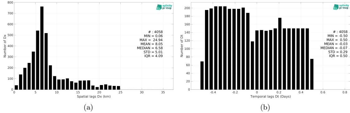
Figure 6: Histograms of the spatial (a) and temporal (b) lags between the location/time of the TSG (Polarstern) measurement and the date of the corresponding SMOS SSS L2 v700 (ESA) SSS pixel.
