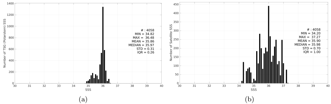
Figure 3: Histograms of SSS from TSG (Polarstern) (a) and SMOS SSS L2 v700 (ESA) (b) considering all match-up pairs per bins of 0.1 over the Amazon and Orinoco river plumes Pi-MEP region and for the full satellite product period.
