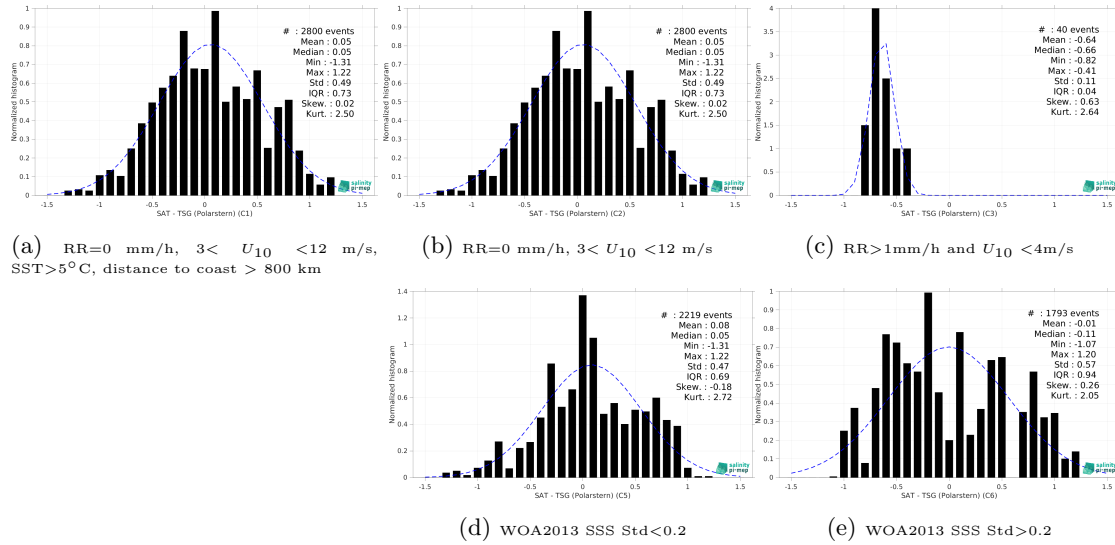
Figure 15: Normalized histogram of \Delta SSS (SMOS SSS L2 v700 (ESA) - TSG (Polarstern)) for 5 different subdatasets corresponding to: RR=0 mm/h, 3 < U_{10} < 12 m/s, SST>5°C, distance to coast > 800 km (a), RR=0 mm/h, 3 < U_{10} < 12 m/s (b), RR>1mm/h and U_{10} < 4 m/s (c), WOA2013 SSS Std<0.2 (d), WOA2013 SSS Std>0.2 (e).
