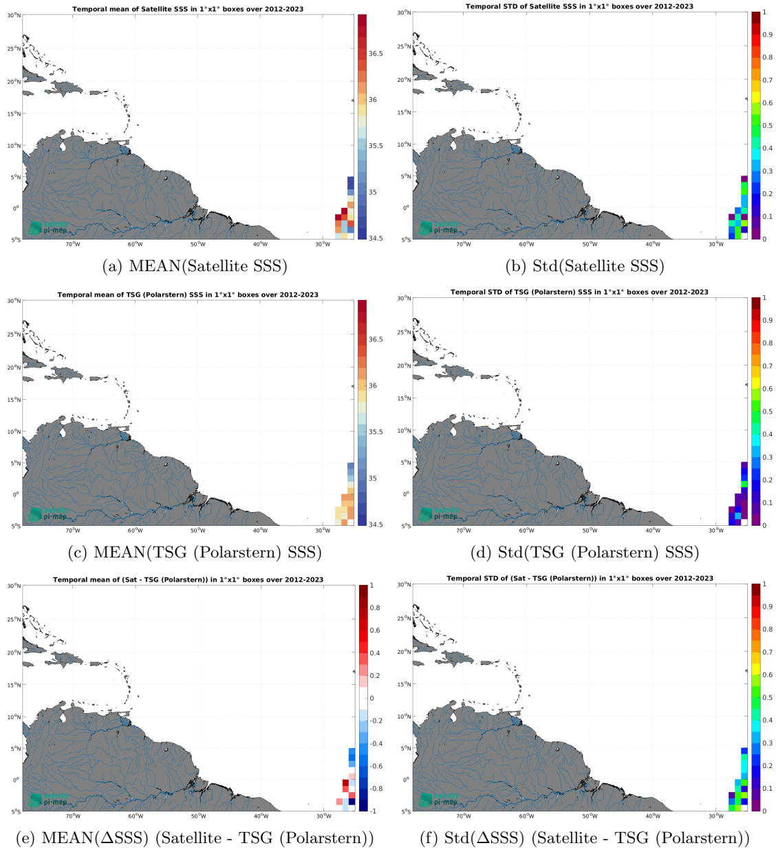
Figure 7: Temporal mean (left) and Std (right) of SSS from SMOS SSS L2 v700 (ESA) (top), TSG (Polarstern) (middle), and of \Delta SSS (Satellite - TSG (Polarstern)). Only match-up pairs are used to generate these maps.
