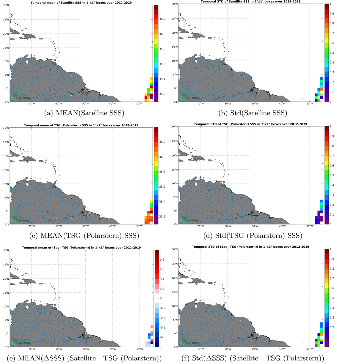
Figure 6: Temporal mean (left) and Std (right) of SSS from SMOS SSS L2 v700 (ESA) (top), TSG (Polarstern) (middle), and of \Delta SSS (Satellite - TSG (Polarstern)). Only match-up pairs are used to generate these maps.
