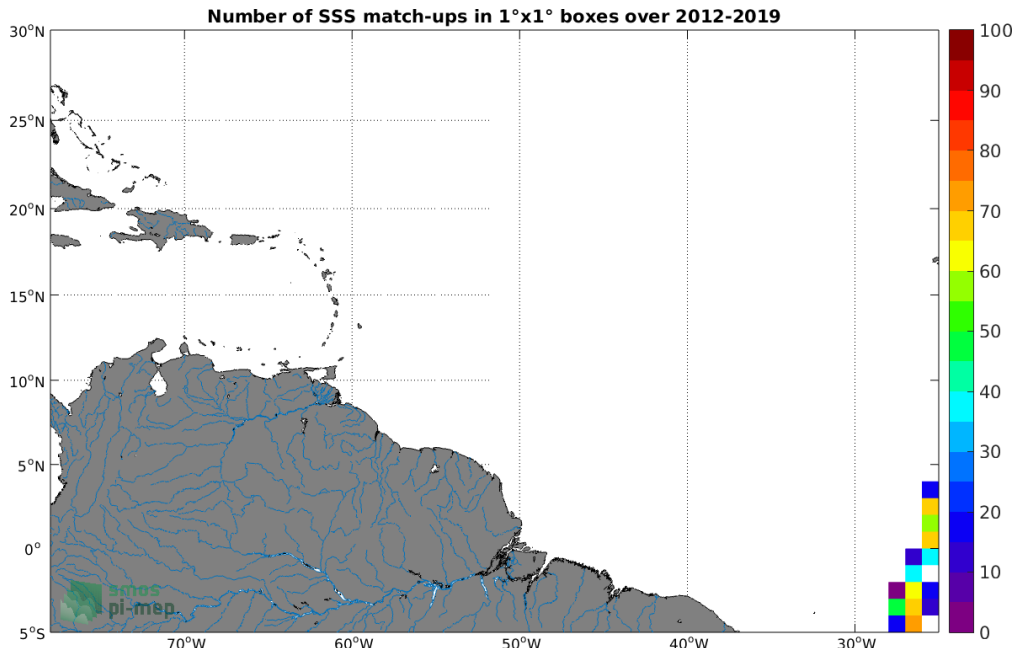
Figure 4: Number of SSS match-ups between TSG (Polarstern) SSS and the SMOS SSS L2 v700 (ESA) SSS product for the Amazon and Orinoco river plumes Pi-MEP region over 1^\circ \times 1^\circ boxes and for the full satellite product period.
