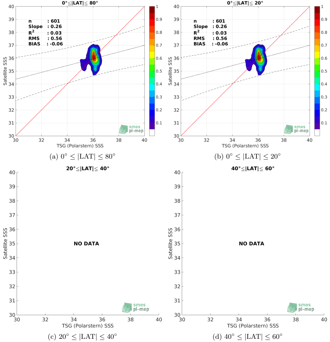
Figure 9: Contour maps of the concentration of SMOS SSS L2 v700 (ESA) SSS (y-axis) versus TSG (Polarstern) SSS (x-axis) at match-up pairs for different latitude bands. For each plot, the red line shows x=y . The black thin and dashed lines indicate a linear fit through the data cloud and the \pm 95\% confidence levels, respectively. The number match-up pairs n , the slope and R^2 coefficient of the linear fit, the root mean square (RMS) and the mean bias between satellite and in situ data are indicated for each latitude band in each plots.
