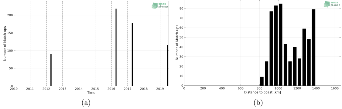
Figure 1: Number of match-ups between TSG (Polarstern) and SMOS SSS L2 v700 (ESA) SSS as a function of time (a) and as function of the distance to coast (b) over the Amazon and Orinoco river plumes Pi-MEP region and for the full satellite product period.
