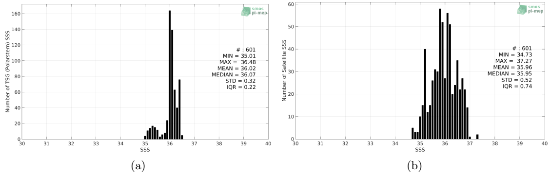
Figure 2: Histograms of SSS from TSG (Polarstern) (a) and SMOS SSS L2 v700 (ESA) (b) considering all match-up pairs per bins of 0.1 over the Amazon and Orinoco river plumes Pi-MEP region and for the full satellite product period.
