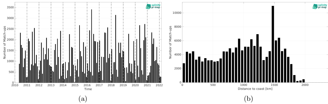
Figure 2: Number of match-ups between TSG (LEGOS-DM) and SMOS SSS L2 v700 (ESA) SSS as a function of time (a) and as function of the distance to coast (b) over the Amazon and Orinoco river plumes Pi-MEP region and for the full satellite product period.
