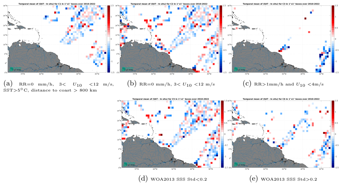
Figure 14: Temporal mean gridded over spatial boxes of size 1^\circ \times 1^\circ of \Delta SSS (SMOS SSS L2 v700 (ESA) - TSG (LEGOS-DM)) for 5 different subdatasets corresponding to:RR=0 mm/h, 3 < U_{10} < 12 m/s, SST >5^\circ\text{C} , distance to coast > 800 km (a), RR=0 mm/h, 3 < U_{10} < 12 m/s (b), RR >1 mm/h and U_{10} < 4 m/s (c), WOA2013 SSS Std <0.2 (d), WOA2013 SSS Std >0.2 (e).
