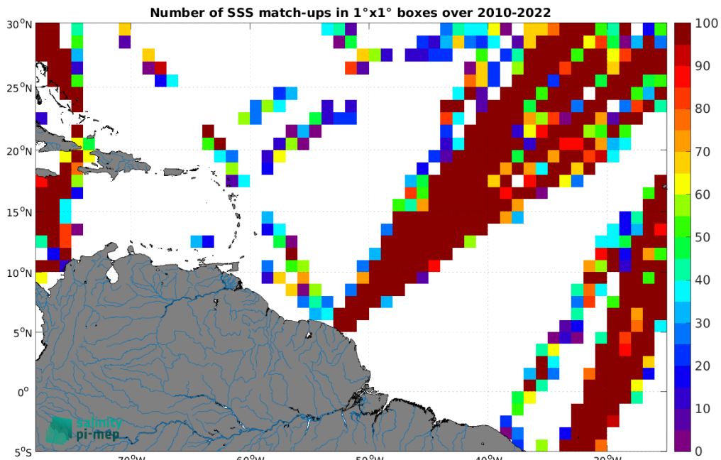
Figure 5: Number of SSS match-ups between TSG (LEGOS-DM) SSS and the SMOS SSS L2 v700 (ESA) SSS product for the Amazon and Orinoco river plumes Pi-MEP region over 1^\circ \times 1^\circ boxes and for the full satellite product period.
