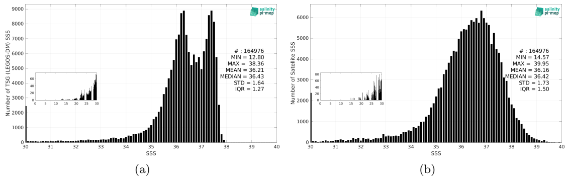
Figure 3: Histograms of SSS from TSG (LEGOS-DM) (a) and SMOS SSS L2 v700 (ESA) (b) considering all match-up pairs per bins of 0.1 over the Amazon and Orinoco river plumes Pi-MEP region and for the full satellite product period.
