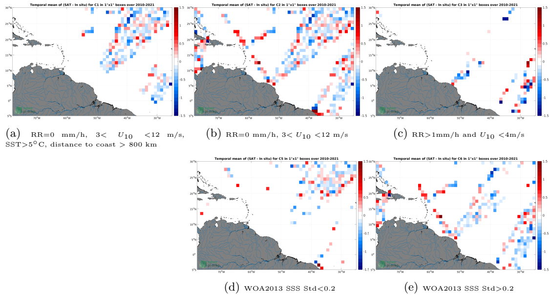
Figure 12: Temporal mean gridded over spatial boxes of size 1^\circ \times 1^\circ of \Delta SSS (SMOS SSS L2 v700 (ESA) - TSG (LEGOS-DM)) for 5 different subdatasets corresponding to:RR=0 mm/h, 3 < U_{10} < 12 m/s, SST >5^\circ\text{C} , distance to coast > 800 km (a), RR=0 mm/h, 3 < U_{10} < 12 m/s (b), RR >1 mm/h and U_{10} < 4 m/s (c), WOA2013 SSS Std <0.2 (d), WOA2013 SSS Std >0.2 (e).
