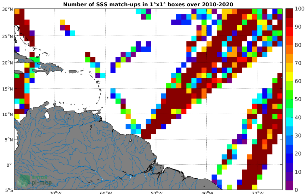
Figure 4: Number of SSS match-ups between TSG (LEGOS-DM) SSS and the SMOS SSS L2 v700 (ESA) SSS product for the Amazon and Orinoco river plumes Pi-MEP region over 1°x1° boxes and for the full satellite product period.
