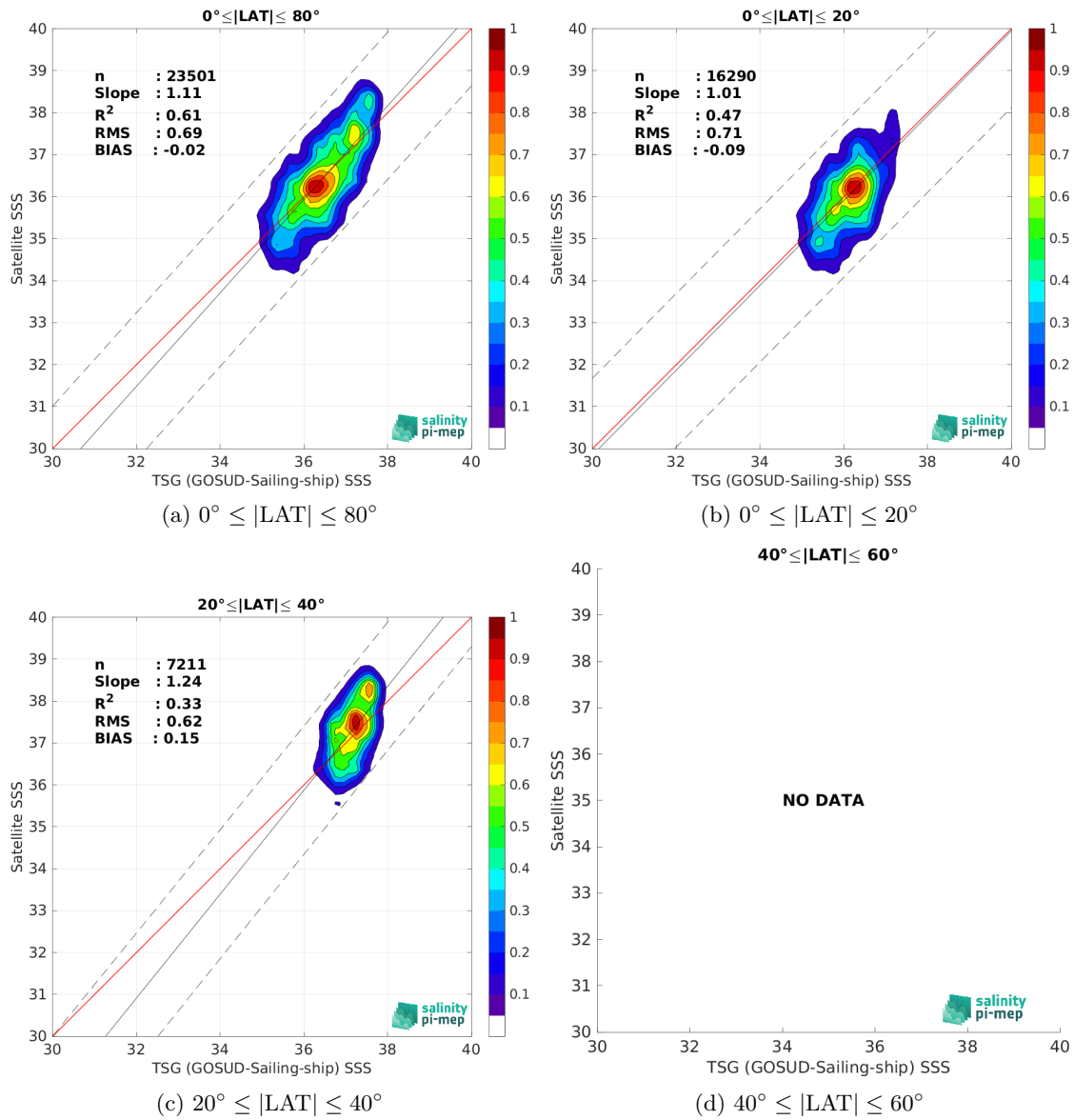
Figure 10: Contour maps of the concentration of SMOS SSS L2 v700 (ESA) SSS (y-axis) versus TSG (GOSUD-Sailing-ship) SSS (x-axis) at match-up pairs for different latitude bands. For each plot, the red line shows x=y . The black thin and dashed lines indicate a linear fit through the data cloud and the \pm 95\% confidence levels, respectively. The number match-up pairs n , the slope and R^2 coefficient of the linear fit, the root mean square (RMS) and the mean bias between satellite and in situ data are indicated for each latitude band in each plots.
