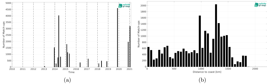
Figure 2: Number of match-ups between TSG (GOSUD-Sailing-ship) and SMOS SSS L2 v700 (ESA) SSS as a function of time (a) and as function of the distance to coast (b) over the Amazon and Orinoco river plumes Pi-MEP region and for the full satellite product period.
