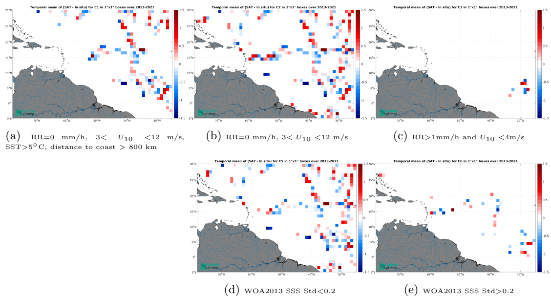
Figure 14: Temporal mean gridded over spatial boxes of size 1^\circ \times 1^\circ of \Delta SSS (SMOS SSS L2 v700 (ESA) - TSG (GOSUD-Sailing-ship)) for 5 different subdatasets corresponding to:RR=0 mm/h, 3 < U_{10} < 12 m/s, SST>5°C, distance to coast > 800 km (a), RR=0 mm/h, 3 < U_{10} < 12 m/s (b), RR>1mm/h and U_{10} < 4 m/s (c), WOA2013 SSS Std<0.2 (d), WOA2013 SSS Std>0.2 (e).
