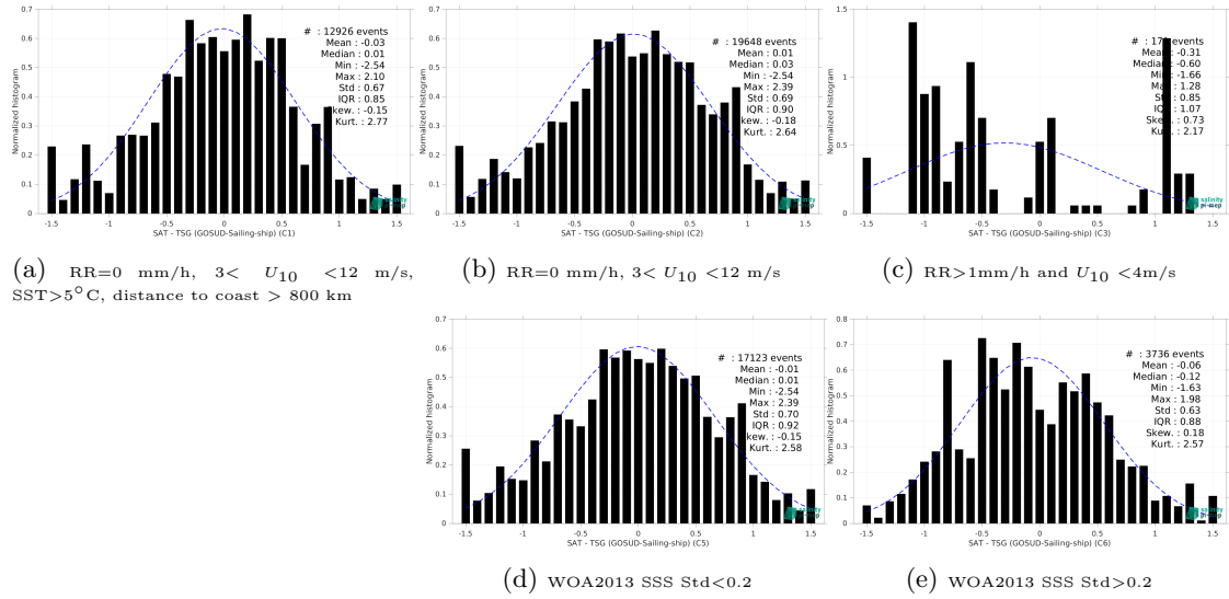
Figure 15: Normalized histogram of \Delta\text{SSS} (SMOS SSS L2 v700 (ESA) - TSG (GOSUD-Sailing-ship)) for 5 different subdatasets corresponding to: RR=0 mm/h, 3 < U_{10} < 12 m/s, SST>5°C, distance to coast > 800 km (a), RR=0 mm/h, 3 < U_{10} < 12 m/s (b), RR>1mm/h and U_{10} < 4 m/s (c), WOA2013 SSS Std<0.2 (d), WOA2013 SSS Std>0.2 (e).
