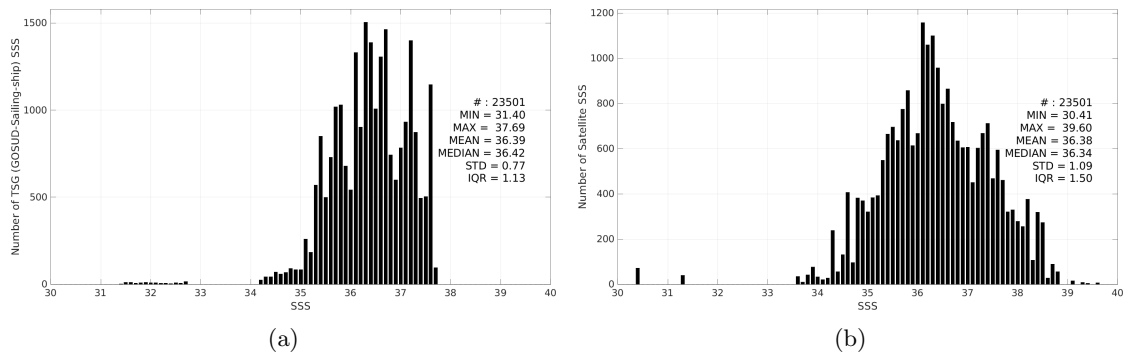
Figure 3: Histograms of SSS from TSG (GOSUD-Sailing-ship) (a) and SMOS SSS L2 v700 (ESA) (b) considering all match-up pairs per bins of 0.1 over the Amazon and Orinoco river plumes Pi-MEP region and for the full satellite product period.
