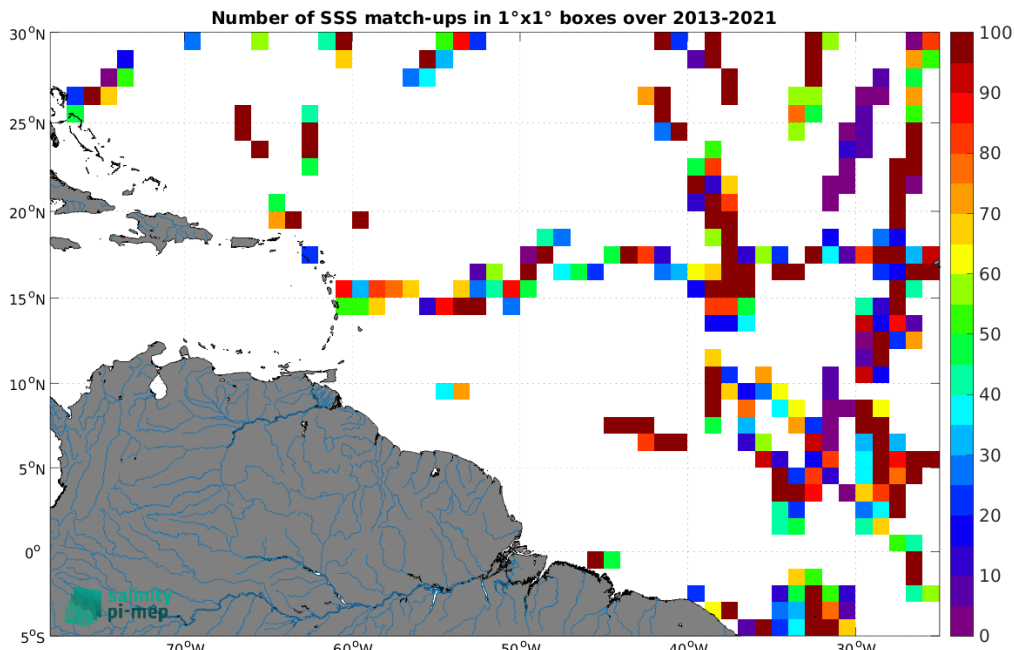
Figure 5: Number of SSS match-ups between TSG (GOSUD-Sailing-ship) SSS and the SMOS SSS L2 v700 (ESA) SSS product for the Amazon and Orinoco river plumes Pi-MEP region over 1^\circ \times 1^\circ boxes and for the full satellite product period.
