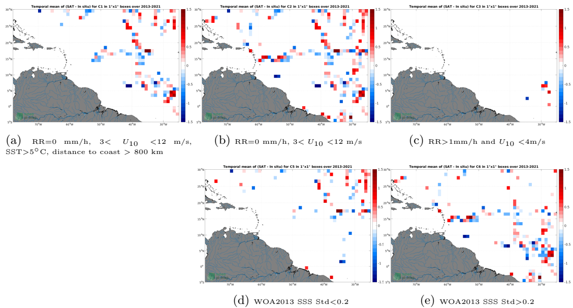
Figure 12: Temporal mean gridded over spatial boxes of size 1^\circ \times 1^\circ of \Delta SSS (SMOS SSS L2 v700 (ESA) - TSG (GOSUD-Sailing-ship)) for 5 different subdatasets corresponding to:RR=0 mm/h, 3 < U_{10} < 12 m/s, SST > 5°C, distance to coast > 800 km (a), RR=0 mm/h, 3 < U_{10} < 12 m/s (b), RR > 1mm/h and U_{10} < 4 m/s (c), WOA2013 SSS Std < 0.2 (d), WOA2013 SSS Std > 0.2 (e).
