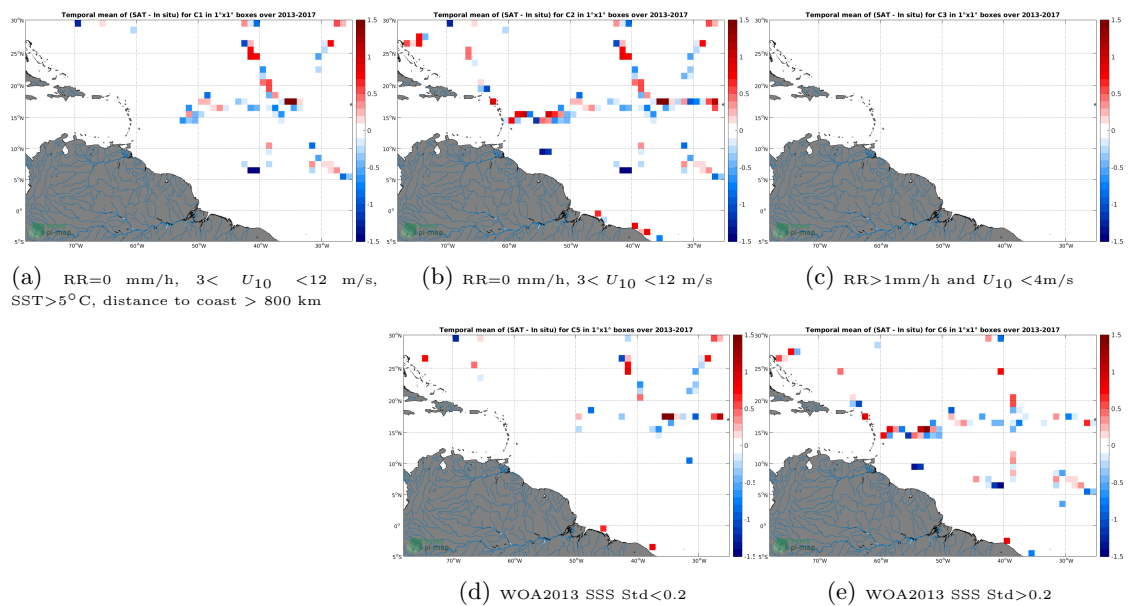
Figure 12: Temporal mean gridded over spatial boxes of size 1°x1° of \Delta SSS (SMOS SSS L2 v700 (ESA) - TSG (GOSUD-Sailing-ship)) for 5 different subdatasets corresponding to:RR=0 mm/h, 3 < U_{10} < 12 m/s, SST>5°C, distance to coast > 800 km (a), RR=0 mm/h, 3 < U_{10} < 12 m/s (b), RR>1mm/h and U_{10} < 4 m/s (c), WOA2013 SSS Std<0.2 (d), WOA2013 SSS Std>0.2 (e).
