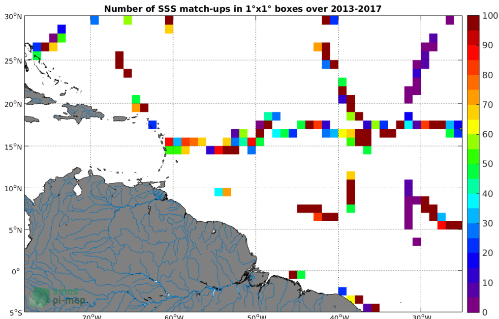
Figure 4: Number of SSS match-ups between TSG (GOSUD-Sailing-ship) SSS and the SMOS SSS L2 v700 (ESA) SSS product for the Amazon and Orinoco river plumes Pi-MEP region over 1°x1° boxes and for the full satellite product period.
