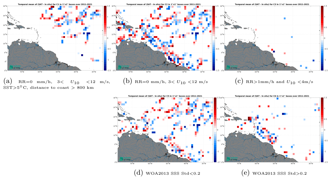
Figure 14: Temporal mean gridded over spatial boxes of size 1^\circ \times 1^\circ of \Delta SSS (SMOS SSS L2 v700 (ESA) - TSG (GOSUD-Research-vessel)) for 5 different subdatasets corresponding to:RR=0 mm/h, 3 < U_{10} < 12 m/s, SST>5°C, distance to coast > 800 km (a), RR=0 mm/h, 3 < U_{10} < 12 m/s (b), RR>1mm/h and U_{10} < 4 m/s (c), WOA2013 SSS Std<0.2 (d), WOA2013 SSS Std>0.2 (e).
