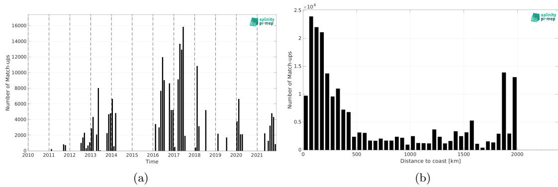
Figure 2: Number of match-ups between TSG (GOSUD-Research-vessel) and SMOS SSS L2 v700 (ESA) SSS as a function of time (a) and as function of the distance to coast (b) over the Amazon and Orinoco river plumes Pi-MEP region and for the full satellite product period.
