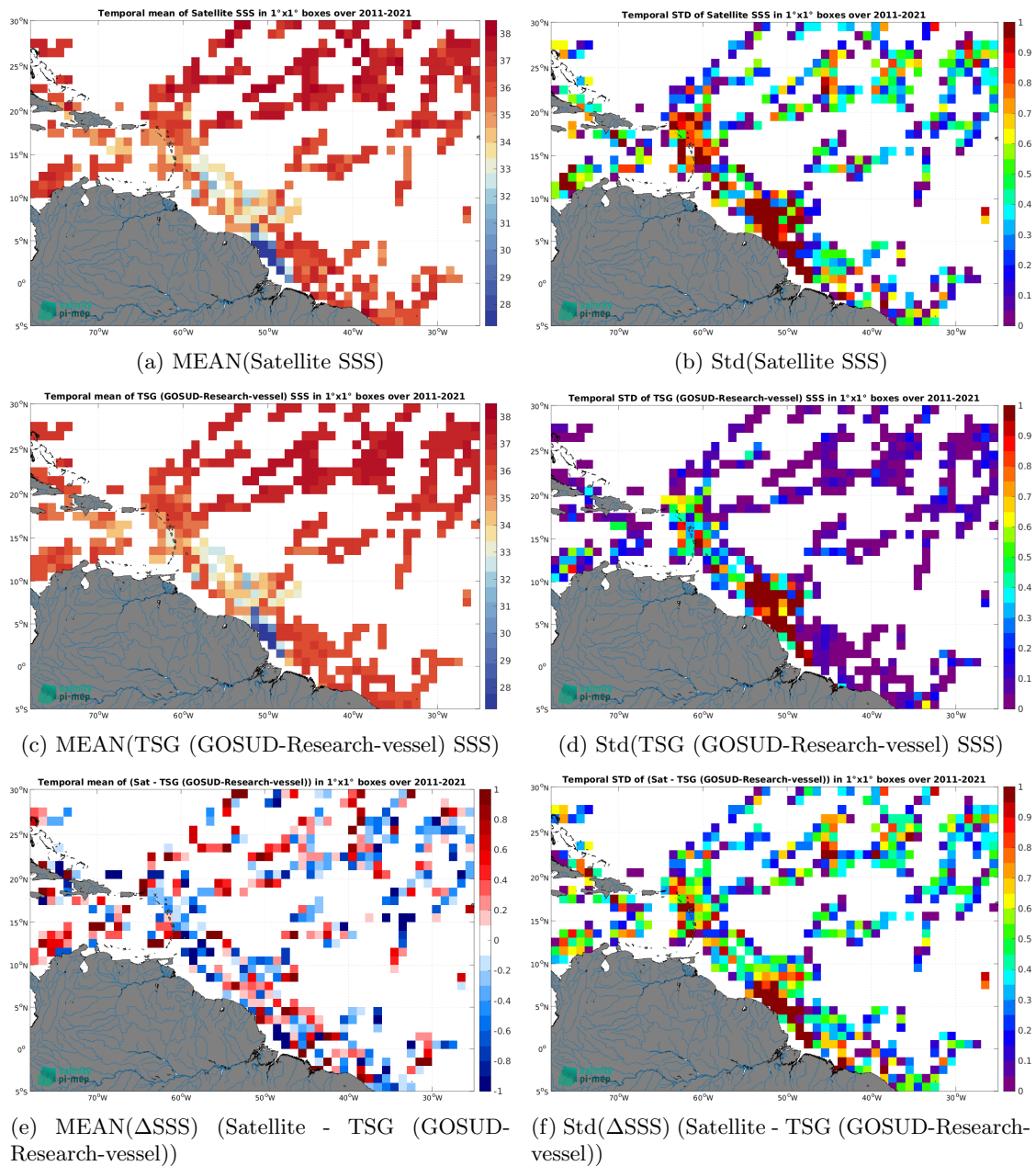
Figure 7: Temporal mean (left) and Std (right) of SSS from SMOS SSS L2 v700 (ESA) (top), TSG (GOSUD-Research-vessel) (middle), and of \Delta SSS (Satellite - TSG (GOSUD-Research-vessel)). Only match-up pairs are used to generate these maps.
