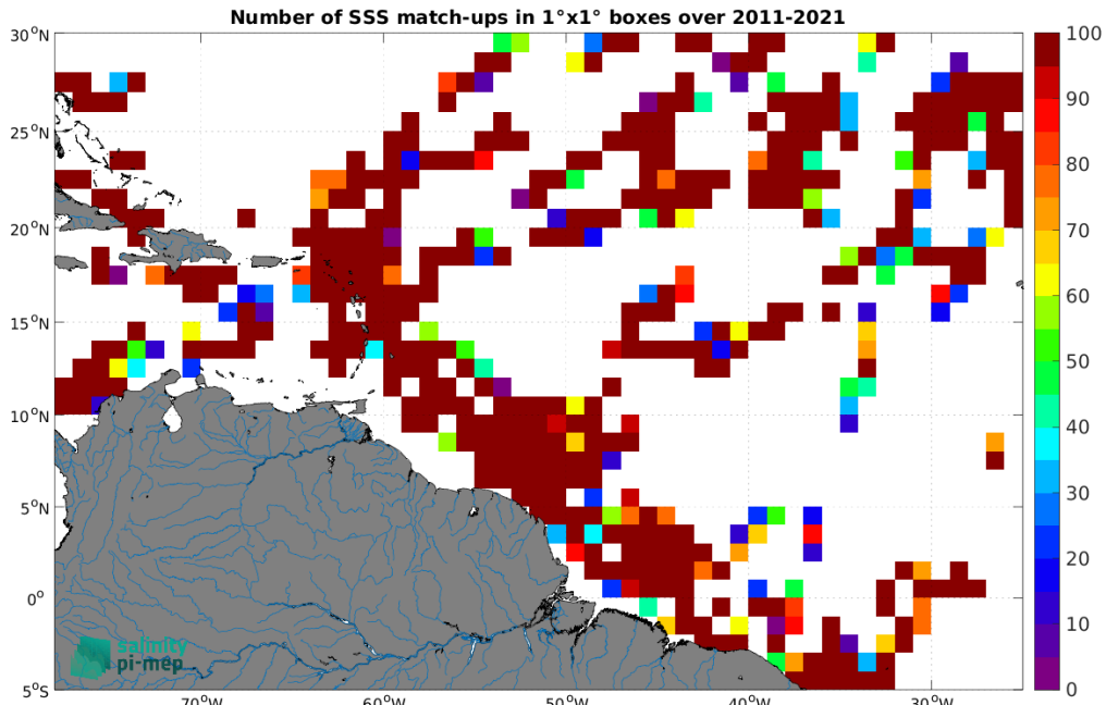
Figure 5: Number of SSS match-ups between TSG (GOSUD-Research-vessel) SSS and the SMOS SSS L2 v700 (ESA) SSS product for the Amazon and Orinoco river plumes Pi-MEP region over 1^\circ \times 1^\circ boxes and for the full satellite product period.
