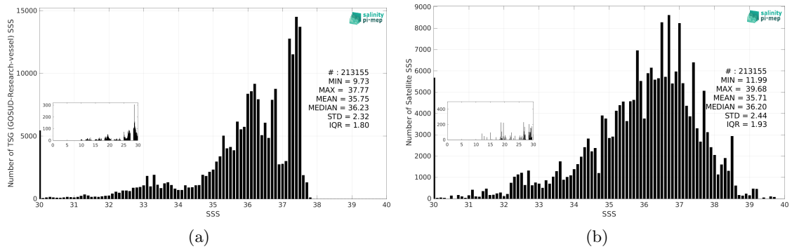
Figure 3: Histograms of SSS from TSG (GOSUD-Research-vessel) (a) and SMOS SSS L2 v700 (ESA) (b) considering all match-up pairs per bins of 0.1 over the Amazon and Orinoco river plumes Pi-MEP region and for the full satellite product period.
