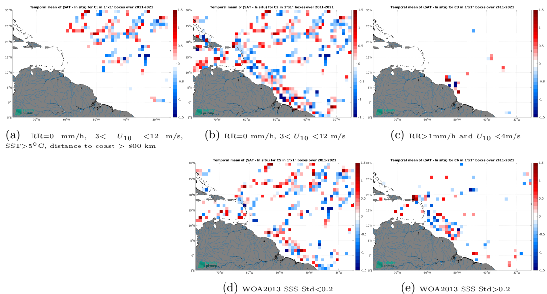
Figure 12: Temporal mean gridded over spatial boxes of size 1^\circ \times 1^\circ of \Delta SSS (SMOS SSS L2 v700 (ESA) - TSG (GOSUD-Research-vessel)) for 5 different subdatasets corresponding to:RR=0 mm/h, 3 < U_{10} < 12 m/s, SST >5^\circ\text{C} , distance to coast > 800 km (a), RR=0 mm/h, 3 < U_{10} < 12 m/s (b), RR >1 mm/h and U_{10} < 4 m/s (c), WOA2013 SSS Std <0.2 (d), WOA2013 SSS Std >0.2 (e).
