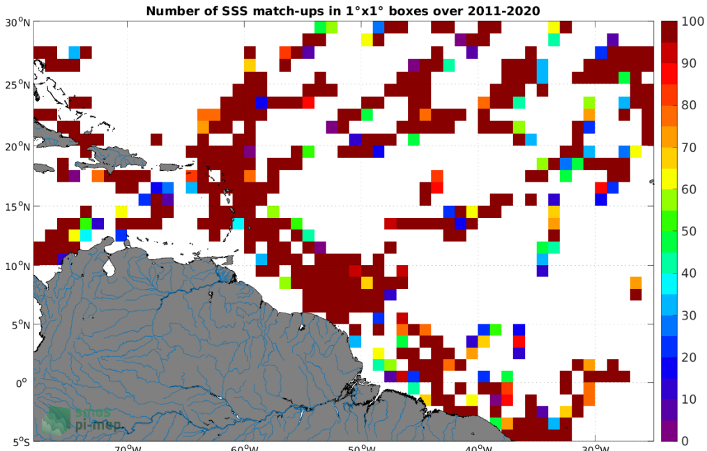
Figure 4: Number of SSS match-ups between TSG (GOSUD-Research-vessel) SSS and the SMOS SSS L2 v700 (ESA) SSS product for the Amazon and Orinoco river plumes Pi-MEP region over 1^{\circ} \times 1^{\circ} boxes and for the full satellite product period.
