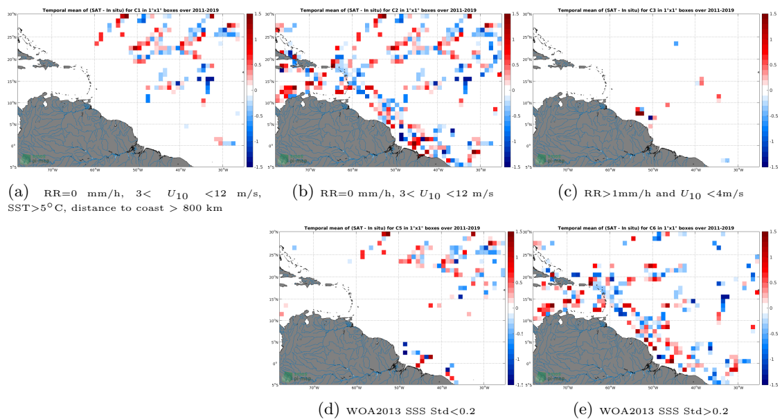
Figure 12: Temporal mean gridded over spatial boxes of size 1°x1° of \Delta SSS (SMOS SSS L2 v700 (ESA) - TSG (GOSUD-Research-vessel)) for 5 different subdatasets corresponding to:RR=0 mm/h, 3 < U_{10} < 12 m/s, SST > 5^{\circ}C , distance to coast > 800 km (a), RR=0 mm/h, 3 < U_{10} < 12 m/s (b), RR>1mm/h and U_{10} < 4 m/s (c), WOA2013 SSS Std<0.2 (d), WOA2013 SSS Std>0.2 (e).
