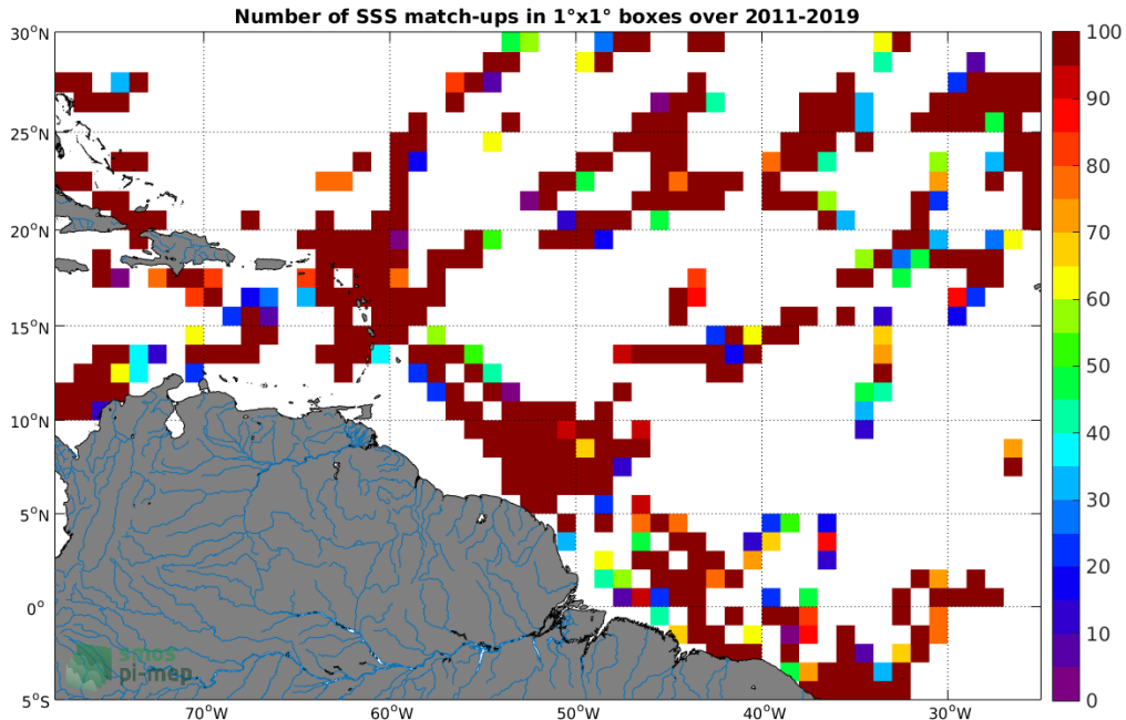
Figure 4: Number of SSS match-ups between TSG (GOSUD-Research-vessel) SSS and the SMOS SSS L2 v700 (ESA) SSS product for the Amazon and Orinoco river plumes Pi-MEP region over 1°x1° boxes and for the full satellite product period.
