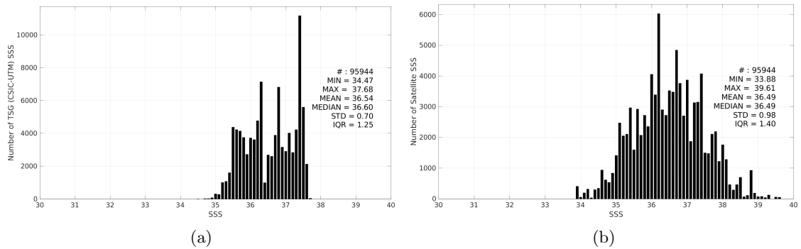
Figure 3: Histograms of SSS from TSG (CSIC-UTM) (a) and SMOS SSS L2 v700 (ESA) (b) considering all match-up pairs per bins of 0.1 over the Amazon and Orinoco river plumes Pi-MEP region and for the full satellite product period.
