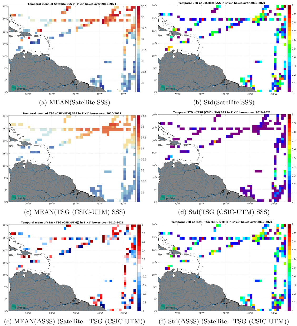
Figure 7: Temporal mean (left) and Std (right) of SSS from SMOS SSS L2 v700 (ESA) (top), TSG (CSIC-UTM) (middle), and of \Delta SSS (Satellite - TSG (CSIC-UTM)). Only match-up pairs are used to generate these maps.
