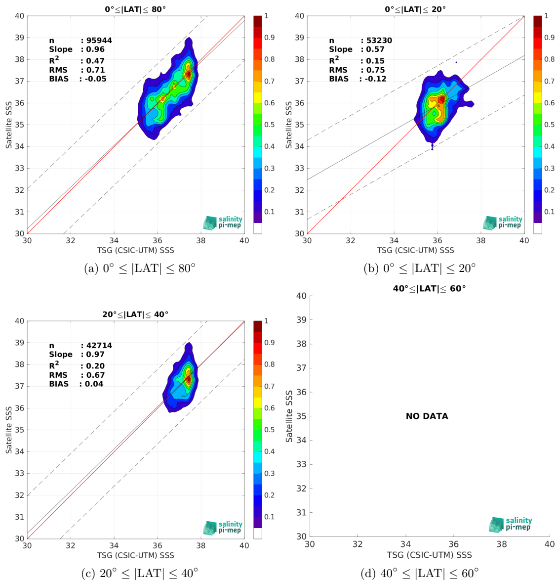
Figure 10: Contour maps of the concentration of SMOS SSS L2 v700 (ESA) SSS (y-axis) versus TSG (CSIC-UTM) SSS (x-axis) at match-up pairs for different latitude bands. For each plot, the red line shows x=y . The black thin and dashed lines indicate a linear fit through the data cloud and the \pm 95\% confidence levels, respectively. The number match-up pairs n , the slope and R^2 coefficient of the linear fit, the root mean square (RMS) and the mean bias between satellite and in situ data are indicated for each latitude band in each plots.
