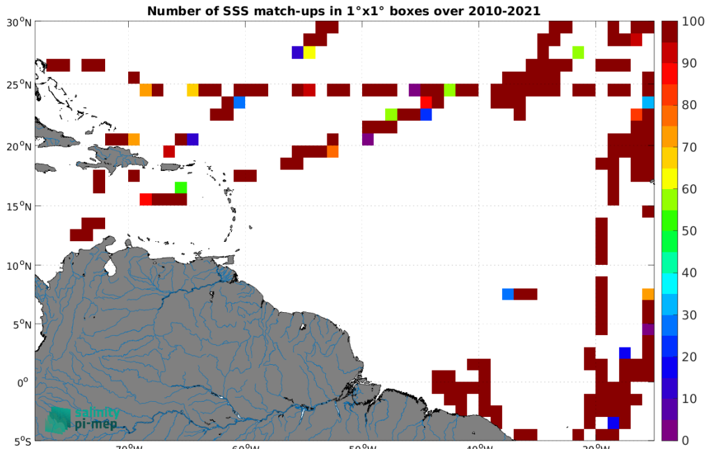
Figure 5: Number of SSS match-ups between TSG (CSIC-UTM) SSS and the SMOS SSS L2 v700 (ESA) SSS product for the Amazon and Orinoco river plumes Pi-MEP region over 1^\circ \times 1^\circ boxes and for the full satellite product period.
