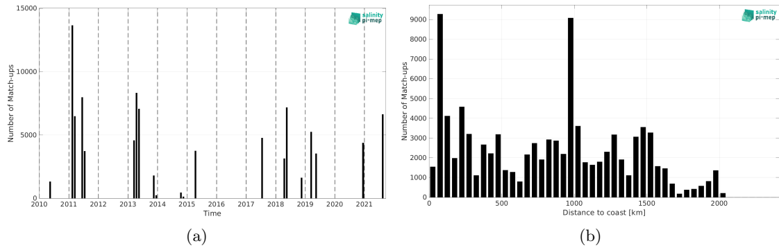
Figure 2: Number of match-ups between TSG (CSIC-UTM) and SMOS SSS L2 v700 (ESA) SSS as a function of time (a) and as function of the distance to coast (b) over the Amazon and Orinoco river plumes Pi-MEP region and for the full satellite product period.
