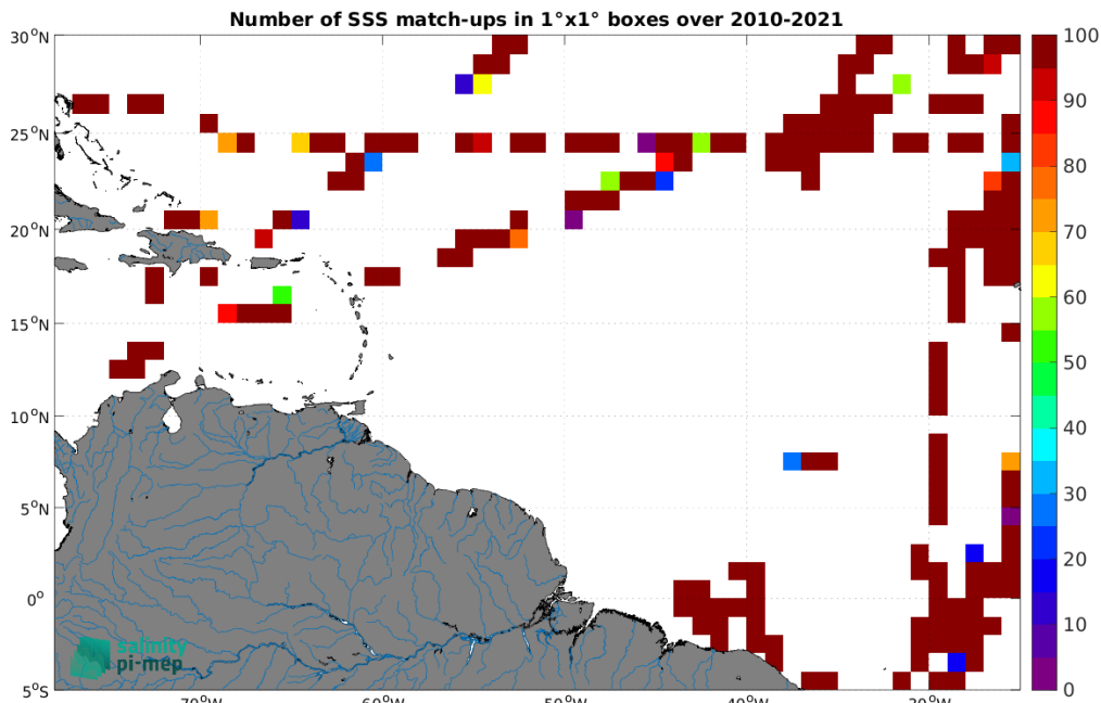
Figure 4: Number of SSS match-ups between TSG (CSIC-UTM) SSS and the SMOS SSS L2 v700 (ESA) SSS product for the Amazon and Orinoco river plumes Pi-MEP region over 1^\circ \times 1^\circ boxes and for the full satellite product period.
