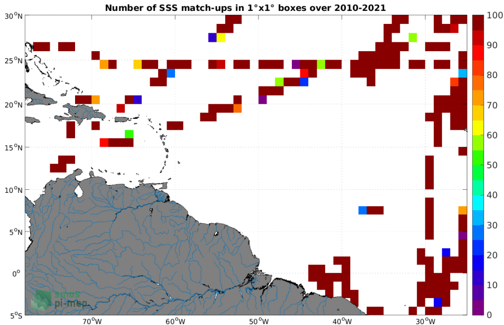
Figure 4: Number of SSS match-ups between TSG (CSIC-UTM) SSS and the SMOS SSS L2 v700 (ESA) SSS product for the Amazon and Orinoco river plumes Pi-MEP region over 1^{\circ} \times 1^{\circ} boxes and for the full satellite product period.
