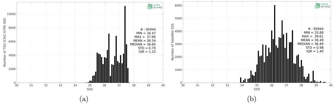
Figure 2: Histograms of SSS from TSG (CSIC-UTM) (a) and SMOS SSS L2 v700 (ESA) (b) considering all match-up pairs per bins of 0.1 over the Amazon and Orinoco river plumes Pi-MEP region and for the full satellite product period.
