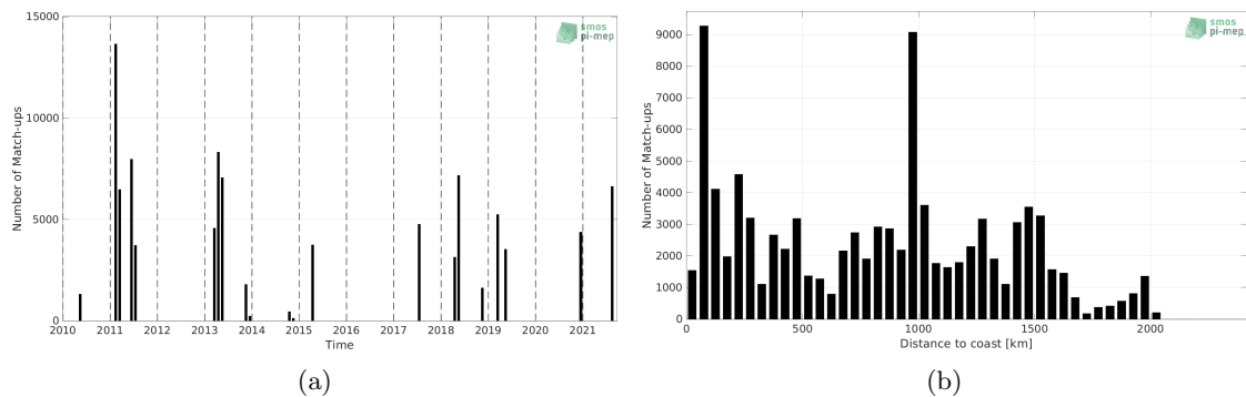
Figure 1: Number of match-ups between TSG (CSIC-UTM) and SMOS SSS L2 v700 (ESA) SSS as a function of time (a) and as function of the distance to coast (b) over the Amazon and Orinoco river plumes Pi-MEP region and for the full satellite product period.
