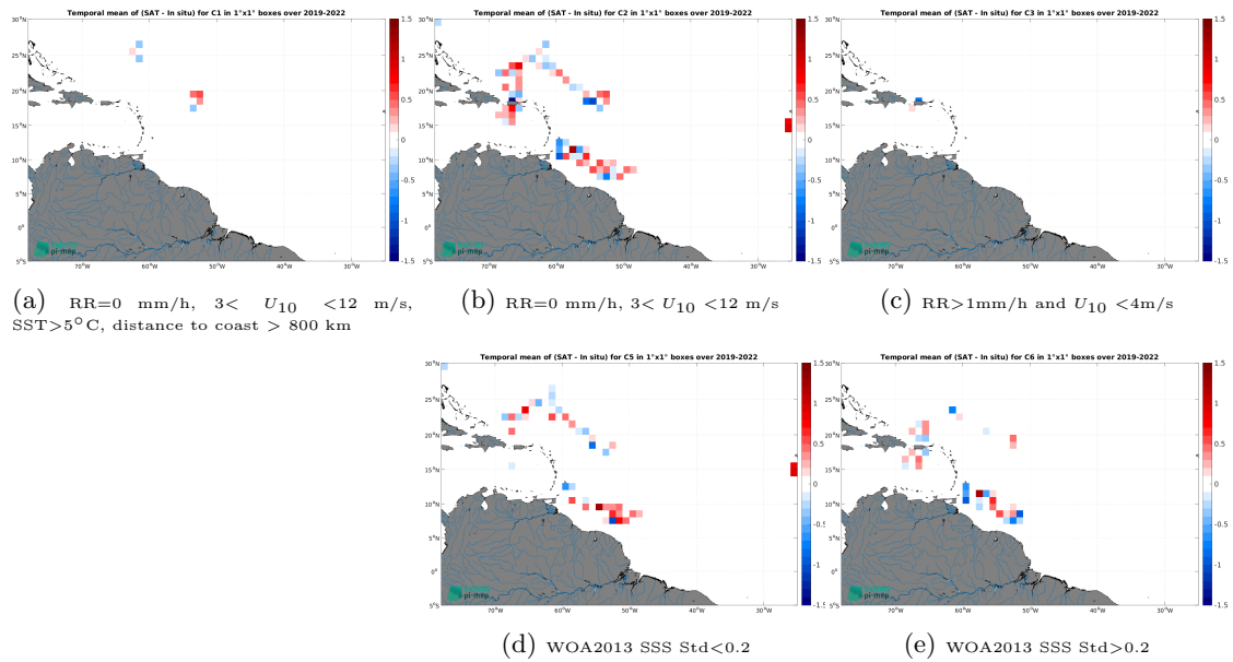
Figure 12: Temporal mean gridded over spatial boxes of size 1^\circ \times 1^\circ of \Delta SSS (SMOS SSS L2 v700 (ESA) - Saildrone) for 5 different subdatasets corresponding to:RR=0 mm/h, 3 < U_{10} < 12 m/s, SST >5^\circ\text{C} , distance to coast > 800 km (a), RR=0 mm/h, 3 < U_{10} < 12 m/s (b), RR >1 mm/h and U_{10} < 4 m/s (c), WOA2013 SSS Std <0.2 (d), WOA2013 SSS Std >0.2 (e).
