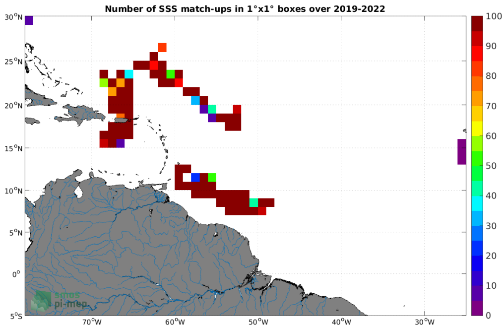
Figure 4: Number of SSS match-ups between Saildrone SSS and the SMOS SSS L2 v700 (ESA) SSS product for the Amazon and Orinoco river plumes Pi-MEP region over 1^\circ \times 1^\circ boxes and for the full satellite product period.
