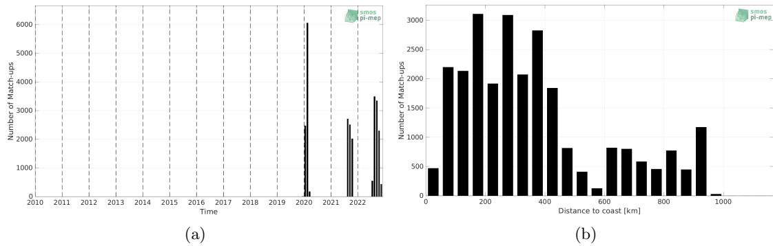
Figure 1: Number of match-ups between Saildrone and SMOS SSS L2 v700 (ESA) SSS as a function of time (a) and as function of the distance to coast (b) over the Amazon and Orinoco river plumes Pi-MEP region and for the full satellite product period.
