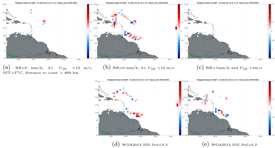
Figure 12: Temporal mean gridded over spatial boxes of size 1^\circ \times 1^\circ of \Delta SSS (SMOS SSS L2 v700 (ESA) - Saldrone) for 5 different subdatasets corresponding to:RR=0 mm/h, 3 < U_{10} < 12 m/s, SST >5^\circ\text{C} , distance to coast > 800 km (a), RR=0 mm/h, 3 < U_{10} < 12 m/s (b), RR >1 mm/h and U_{10} < 4 m/s (c), WOA2013 SSS Std <0.2 (d), WOA2013 SSS Std >0.2 (e).
