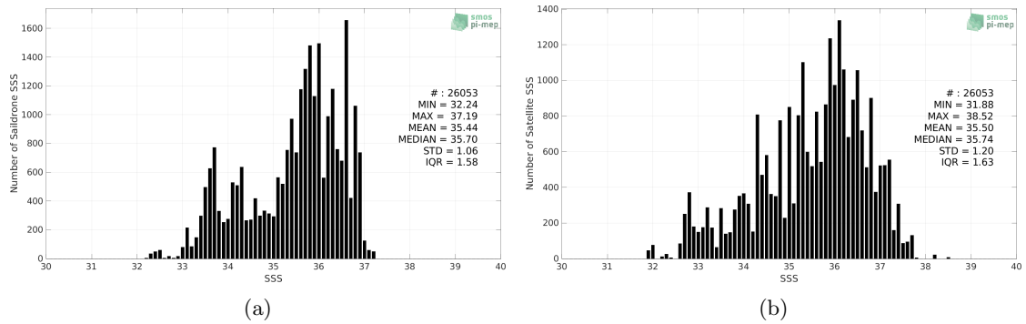
Figure 2: Histograms of SSS from Saildrone (a) and SMOS SSS L2 v700 (ESA) (b) considering all match-up pairs per bins of 0.1 over the Amazon and Orinoco river plumes Pi-MEP region and for the full satellite product period.
