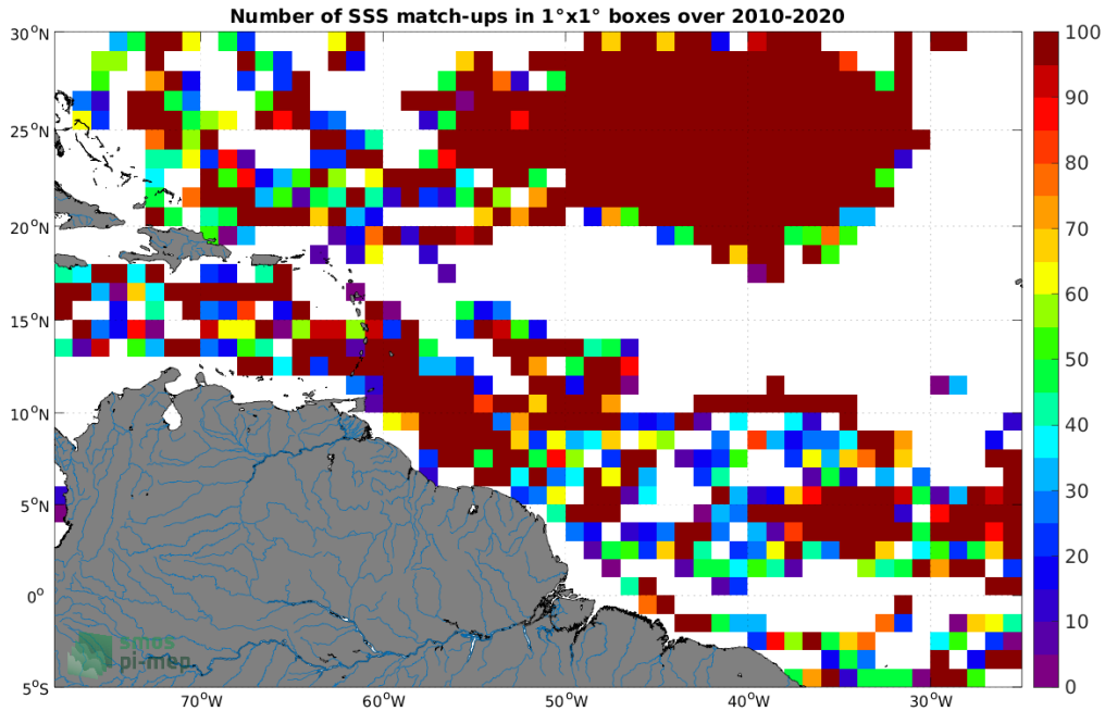
Figure 3: Number of SSS match-ups between Surface drifters SSS and the SMOS SSS L2 v700 (ESA) SSS product for the Amazon and Orinoco river plumes Pi-MEP region over 1^{\circ} \times 1^{\circ} boxes and for the full satellite product period.
