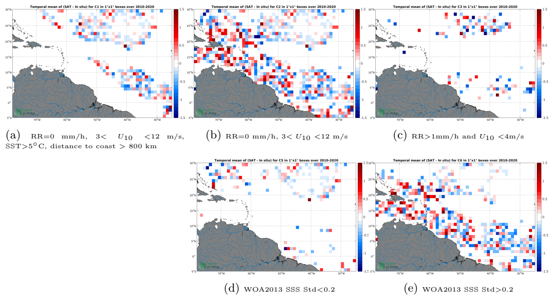
Figure 11: Temporal mean gridded over spatial boxes of size 1°x1° of \Delta SSS (SMOS SSS L2 v700 (ESA) - Surface drifters) for 5 different subdatasets corresponding to:RR=0 mm/h, 3 < U_{10} < 12 m/s, SST>5°C, distance to coast > 800 km (a), RR=0 mm/h, 3 < U_{10} < 12 m/s (b), RR>1mm/h and U_{10} < 4 m/s (c), WOA2013 SSS Std<0.2 (d), WOA2013 SSS Std>0.2 (e).
