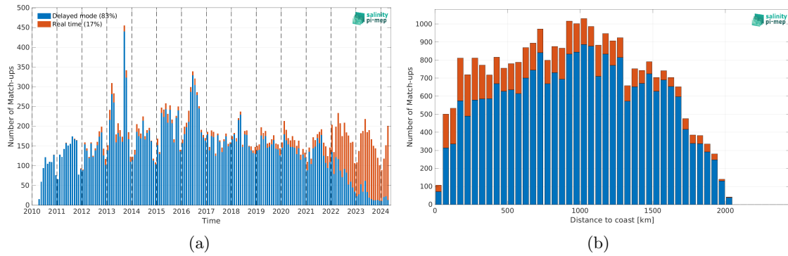
Figure 2: Number of match-ups between Argo and SMOS SSS L2 v700 (ESA) SSS as a function of time (a) and as function of the distance to coast (b) over the Amazon and Orinoco river plumes Pi-MEP region and for the full satellite product period.
