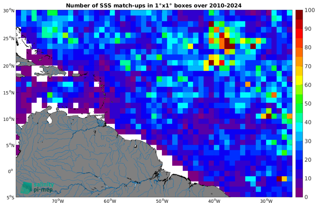
Figure 5: Number of SSS match-ups between Argo SSS and the SMOS SSS L2 v700 (ESA) SSS product for the Amazon and Orinoco river plumes Pi-MEP region over 1^\circ \times 1^\circ boxes and for the full satellite product period.
