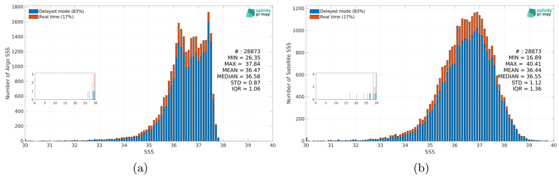
Figure 3: Histograms of SSS from Argo (a) and SMOS SSS L2 v700 (ESA) (b) considering all match-up pairs per bins of 0.1 over the Amazon and Orinoco river plumes Pi-MEP region and for the full satellite product period.
