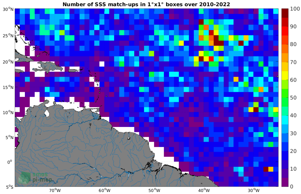
Figure 4: Number of SSS match-ups between Argo SSS and the SMOS SSS L2 v700 (ESA) SSS product for the Amazon and Orinoco river plumes Pi-MEP region over 1^{\circ} \times 1^{\circ} boxes and for the full satellite product period.
