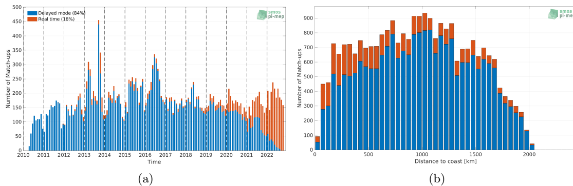
Figure 1: Number of match-ups between Argo and SMOS SSS L2 v700 (ESA) SSS as a function of time (a) and as function of the distance to coast (b) over the Amazon and Orinoco river plumes Pi-MEP region and for the full satellite product period.
