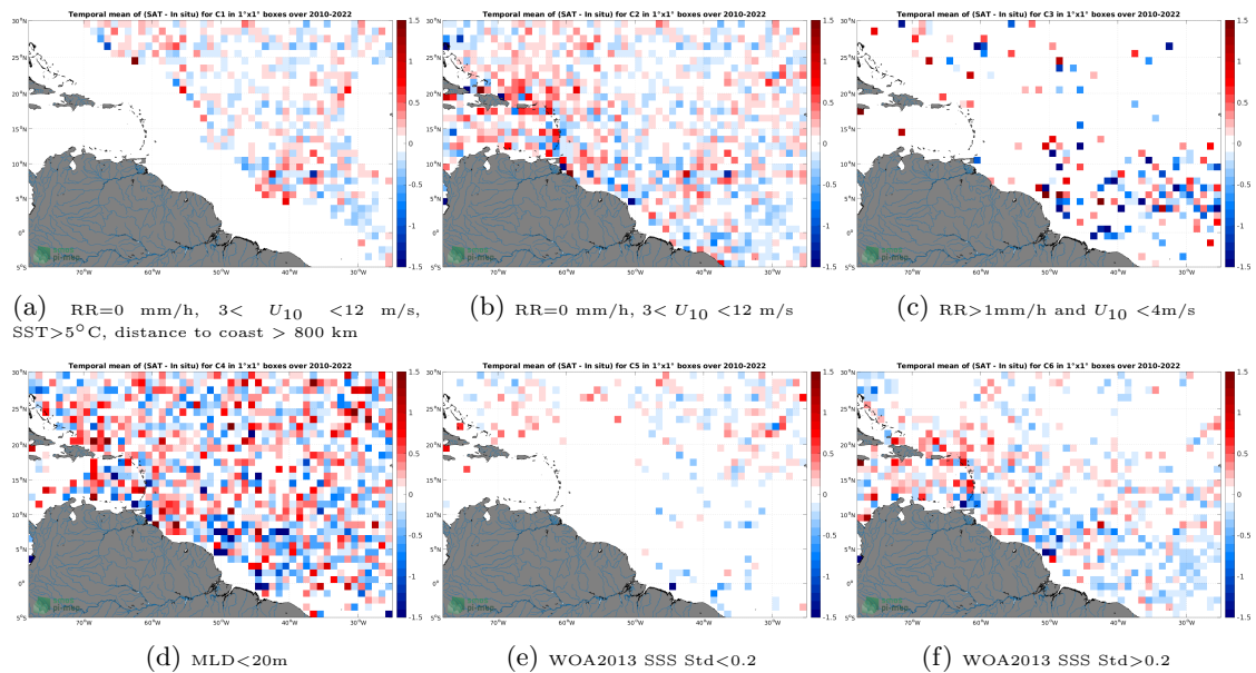
Figure 12: Temporal mean gridded over spatial boxes of size 1^\circ \times 1^\circ of \Delta SSS (SMOS SSS L2 v700 (ESA) - Argo) for 6 different subdatasets corresponding to: RR=0 mm/h, 3 < U_{10} < 12 m/s, SST > 5^\circ\text{C} , distance to coast > 800 km (a), RR=0 mm/h, 3 < U_{10} < 12 m/s (b), RR > 1 mm/h and U_{10} < 4 m/s (c),MLD < 20 m (d),WOA2013 SSS Std < 0.2 (e),WOA2013 SSS Std > 0.2 (f).
