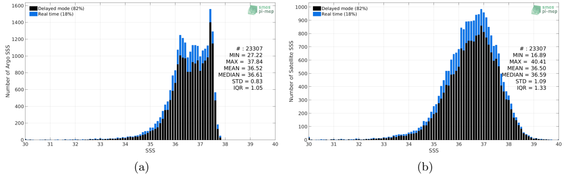
Figure 2: Histograms of SSS from Argo (a) and SMOS SSS L2 v700 (ESA) (b) considering all match-up pairs per bins of 0.1 over the Amazon and Orinoco river plumes Pi-MEP region and for the full satellite product period.
