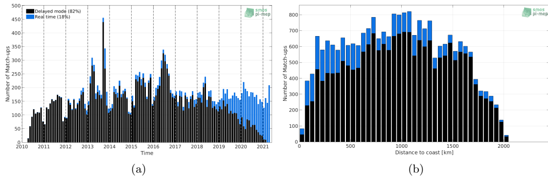
Figure 1: Number of match-ups between Argo and SMOS SSS L2 v700 (ESA) SSS as a function of time (a) and as function of the distance to coast (b) over the Amazon and Orinoco river plumes Pi-MEP region and for the full satellite product period.
