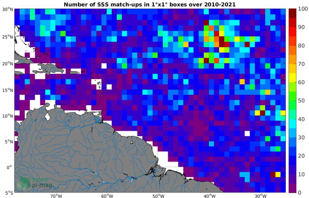
Figure 4: Number of SSS match-ups between Argo SSS and the SMOS SSS L2 v700 (ESA) SSS product for the Amazon and Orinoco river plumes Pi-MEP region over 1°x1° boxes and for the full satellite product period.
