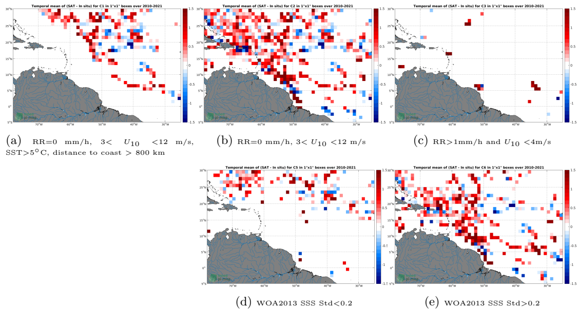
Figure 12: Temporal mean gridded over spatial boxes of size 1^\circ \times 1^\circ of \Delta SSS (SMOS SSS L2 v662 (ESA) - TSG (SAMOS)) for 5 different subdatasets corresponding to:RR=0 mm/h, 3 < U_{10} < 12 m/s, SST >5^\circ\text{C} , distance to coast > 800 km (a), RR=0 mm/h, 3 < U_{10} < 12 m/s (b), RR >1 mm/h and U_{10} < 4 m/s (c), WOA2013 SSS Std <0.2 (d), WOA2013 SSS Std >0.2 (e).
