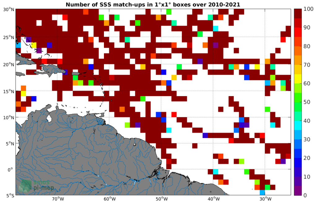
Figure 4: Number of SSS match-ups between TSG (SAMOS) SSS and the SMOS SSS L2 v662 (ESA) SSS product for the Amazon and Orinoco river plumes Pi-MEP region over 1^{\circ} \times 1^{\circ} boxes and for the full satellite product period.
