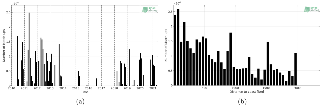
Figure 1: Number of match-ups between TSG (SAMOS) and SMOS SSS L2 v662 (ESA) SSS as a function of time (a) and as function of the distance to coast (b) over the Amazon and Orinoco river plumes Pi-MEP region and for the full satellite product period.
