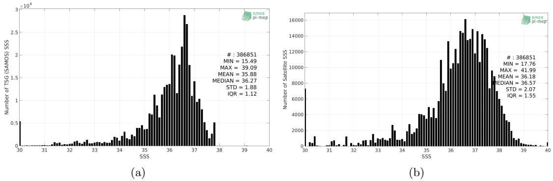
Figure 2: Histograms of SSS from TSG (SAMOS) (a) and SMOS SSS L2 v662 (ESA) (b) considering all match-up pairs per bins of 0.1 over the Amazon and Orinoco river plumes Pi-MEP region and for the full satellite product period.
