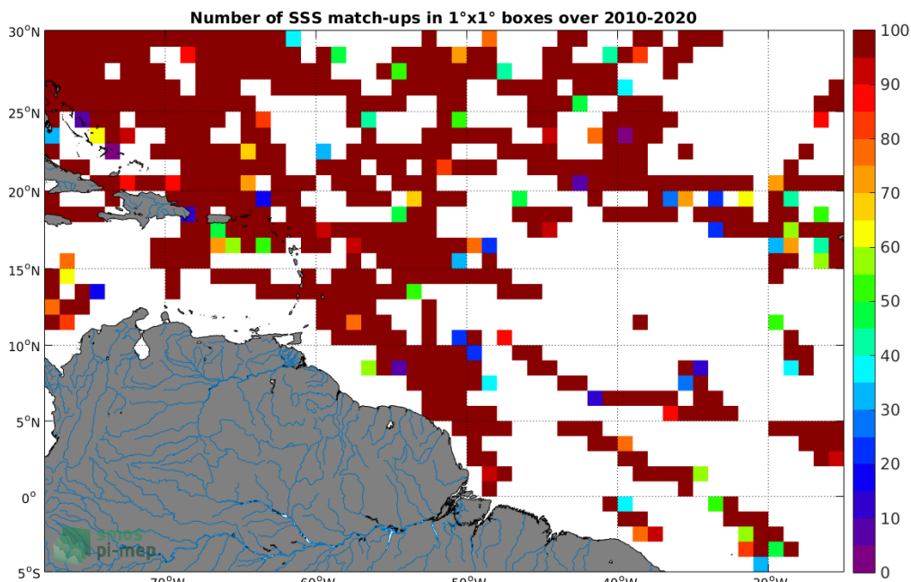
Figure 4: Number of SSS match-ups between TSG (SAMOS) SSS and the SMOS SSS L2 v662 (ESA) SSS product for the Amazon and Orinoco river plumes Pi-MEP region over 1°x1° boxes and for the full satellite product period.
