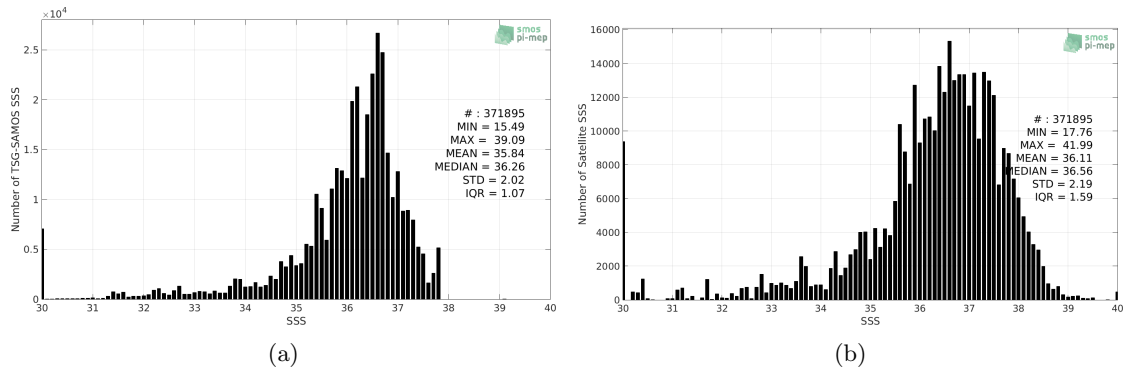
Figure 2: Histograms of SSS from TSG-SAMOS (a) and SMOS L2 v662 (ESA) (b) considering all match-up pairs per bins of 0.1 over the Amazon and Orinoco river plumes Pi-MEP region and for the full satellite product period.
