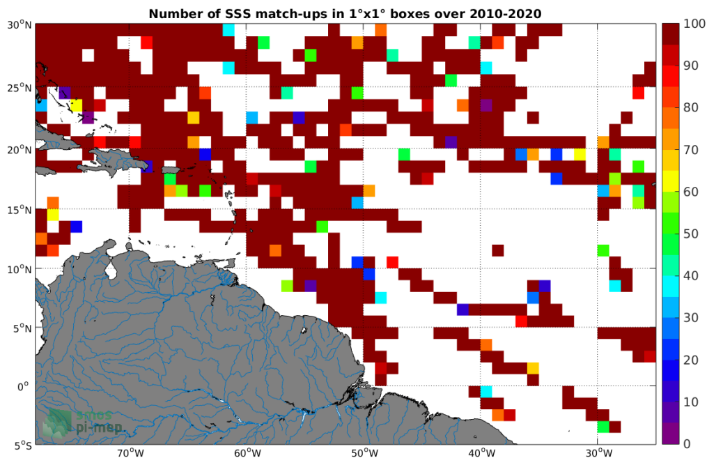
Figure 4: Number of SSS match-ups between TSG-SAMOS SSS and the SMOS L2 v662 (ESA) SSS product for the Amazon and Orinoco river plumes Pi-MEP region over 1^\circ \times 1^\circ boxes and for the full satellite product period.
