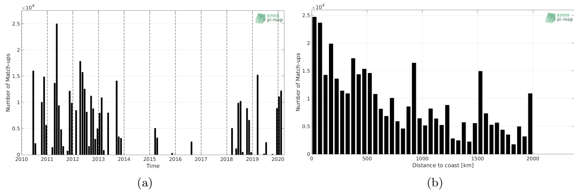
Figure 1: Number of match-ups between TSG-SAMOS and SMOS L2 v662 (ESA) SSS as a function of time (a) and as function of the distance to coast (b) over the Amazon and Orinoco river plumes Pi-MEP region and for the full satellite product period.
