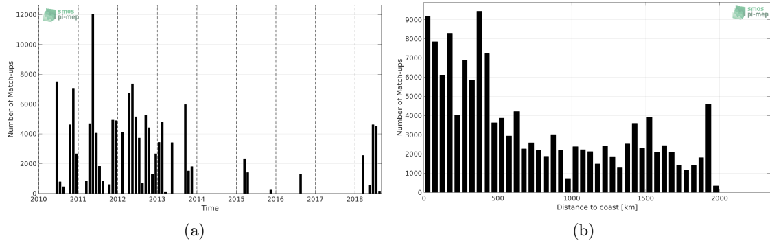
Figure 1: Number of match-ups between TSG-SAMOS and SMOS-L2-DPGS-v662 SSS as a function of time (a) and as function of the distance to coast (b) over the Amazon and Orinoco river plumes Pi-MEP region and for the full satellite product period.
