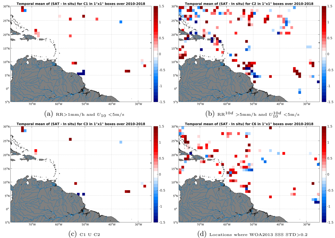
Figure 12: Temporal mean gridded over spatial boxes of size 1^\circ \times 1^\circ of \Delta SSS (SMOS-L2-DPGS-v662 - TSG-SAMOS) for 4 different subdatasets corresponding to: RR > 1mm/h and U_{10} < 5 m/s (a), RR^{10d} > 5 mm/h and U_{10}^{10d} < 5 m/s (b), C1 U C2 (c), Locations where WOA2013 SSS STD > 0.2 (d).
