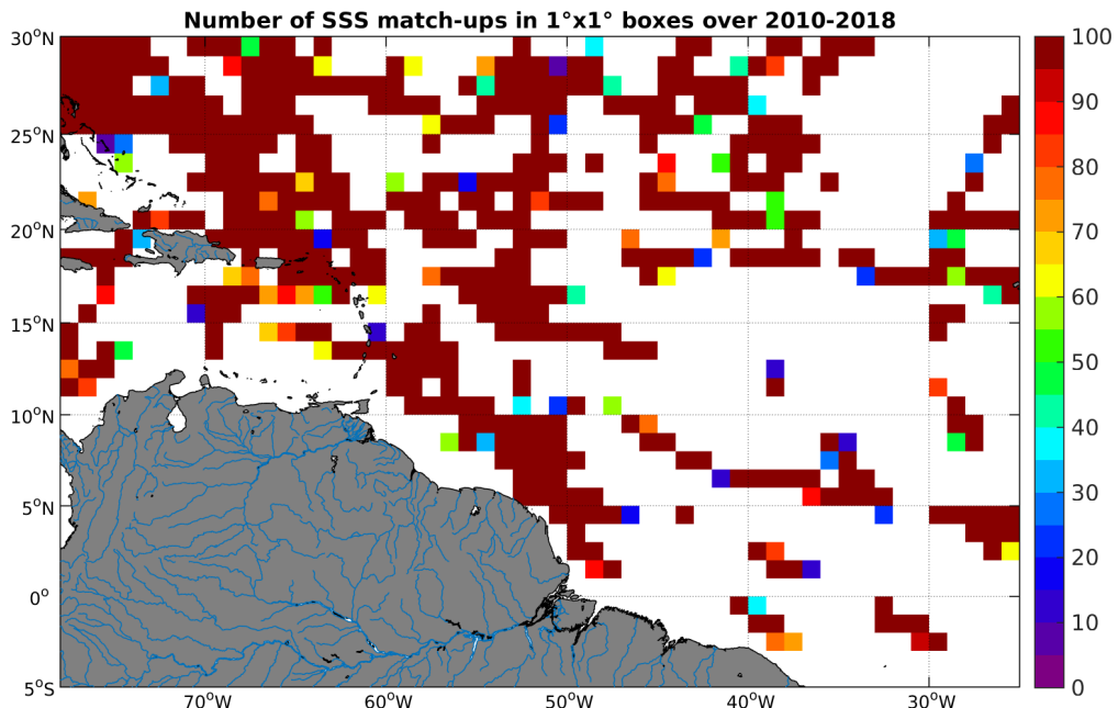
Figure 4: Number of SSS match-ups between TSG-SAMOS SSS and the SMOS-L2-DPGS-v662 SSS product for the Amazon and Orinoco river plumes Pi-MEP region over 1^\circ \times 1^\circ boxes and for the full satellite product period.
