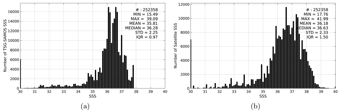
Figure 2: Histograms of SSS from TSG-SAMOS (a) and SMOS-L2-DPGS-v662 (b) considering all match-up pairs per bins of 0.1 over the Amazon and Orinoco river plumes Pi-MEP region and for the full satellite product period.
