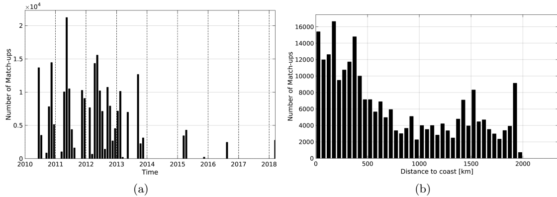
Figure 1: Number of match-ups between TSG-SAMOS and SMOS-L2-DPGS-v662 SSS as a function of time (a) and as function of the distance to coast (b) over the Amazon and Orinoco river plumes Pi-MEP region and for the full satellite product period.
