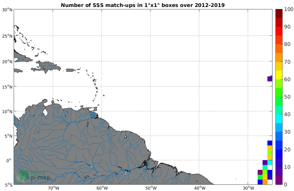
Figure 4: Number of SSS match-ups between TSG-POLARSTERN SSS and the SMOS L2 v662 (ESA) SSS product for the Amazon and Orinoco river plumes Pi-MEP region over 1^\circ \times 1^\circ boxes and for the full satellite product period.
