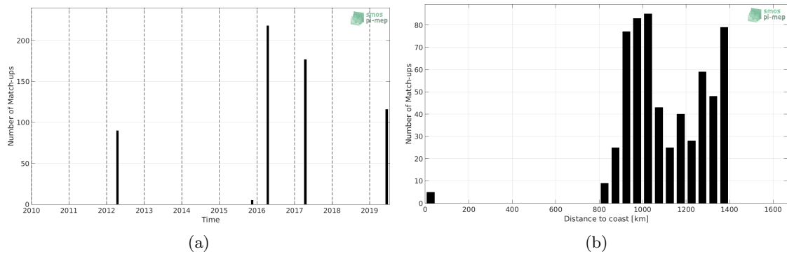
Figure 1: Number of match-ups between TSG-POLARSTERN and SMOS L2 v662 (ESA) SSS as a function of time (a) and as function of the distance to coast (b) over the Amazon and Orinoco river plumes Pi-MEP region and for the full satellite product period.
