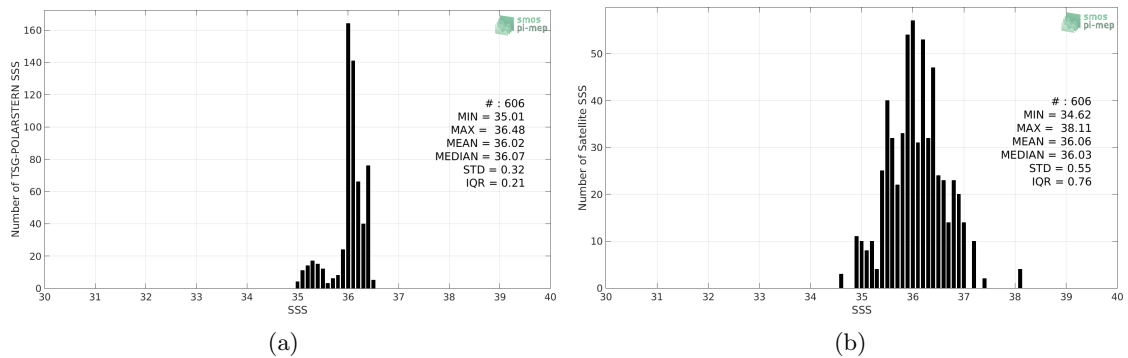
Figure 2: Histograms of SSS from TSG-POLARSTERN (a) and SMOS L2 v662 (ESA) (b) considering all match-up pairs per bins of 0.1 over the Amazon and Orinoco river plumes Pi-MEP region and for the full satellite product period.
