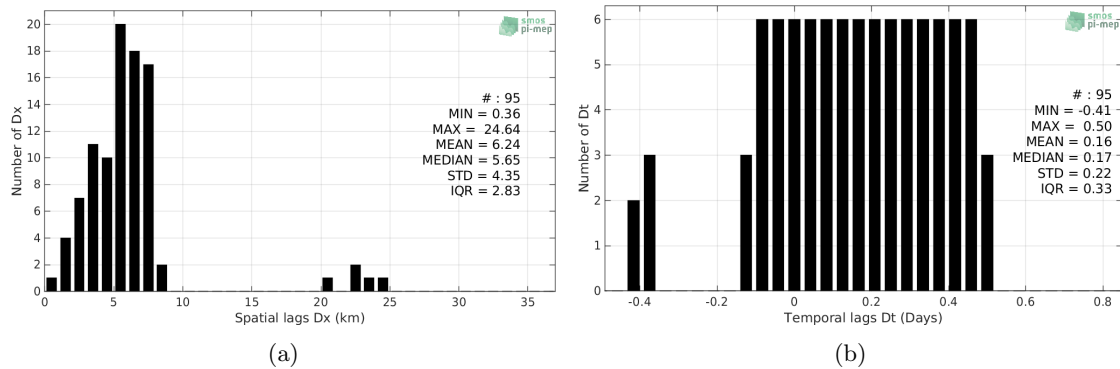
Figure 5: Histograms of the spatial (a) and temporal (b) lags between the time of the TSG-POLARSTERN measurements and the date of the corresponding SMOS-L2-DPGS-v662 SSS product.
