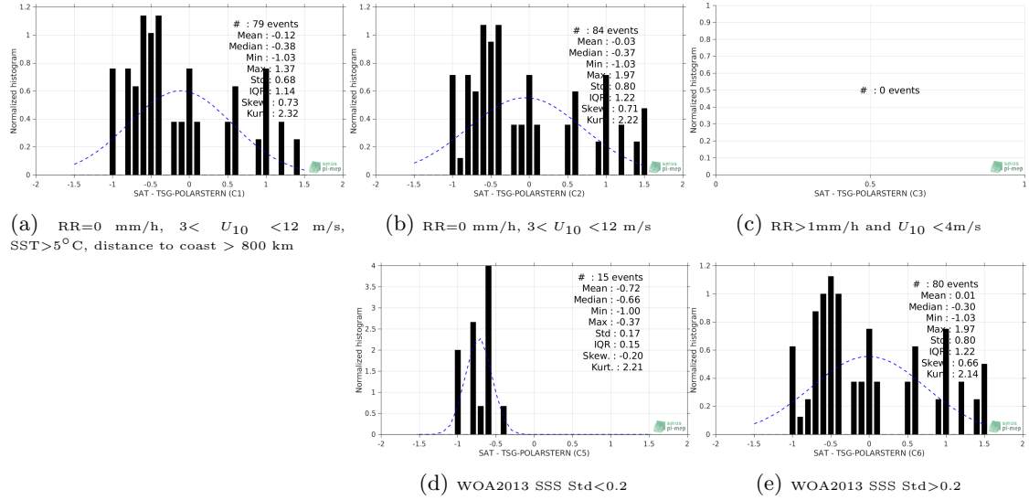
Figure 13: Normalized histogram of \Delta SSS (SMOS-L2-DPGS-v662 - TSG-POLARSTERN) for 5 different subdatasets corresponding to: RR=0 mm/h, 3 < U_{10} < 12 m/s, SST > 5°C, distance to coast > 800 km (a), RR=0 mm/h, 3 < U_{10} < 12 m/s (b), RR > 1mm/h and U_{10} < 4 m/s (c), WOA2013 SSS Std < 0.2 (d), WOA2013 SSS Std > 0.2 (e).
