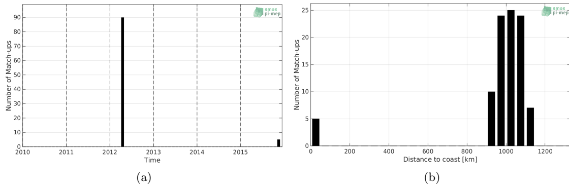
Figure 1: Number of match-ups between TSG-POLARSTERN and SMOS-L2-DPGS-v662 SSS as a function of time (a) and as function of the distance to coast (b) over the Amazon and Orinoco river plumes Pi-MEP region and for the full satellite product period.
