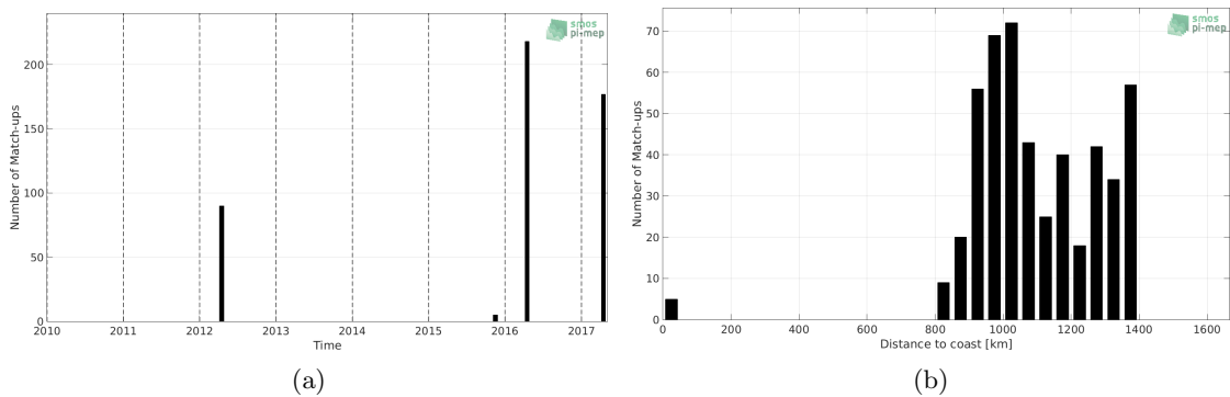
Figure 1: Number of match-ups between TSG-POLARSTERN and SMOS-L2-DPGS-v662 SSS as a function of time (a) and as function of the distance to coast (b) over the Amazon and Orinoco river plumes Pi-MEP region and for the full satellite product period.
