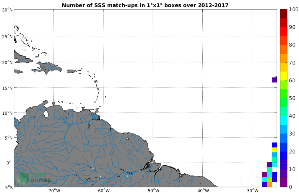
Figure 4: Number of SSS match-ups between TSG-POLARSTERN SSS and the SMOS-L2-DPGS-v662 SSS product for the Amazon and Orinoco river plumes Pi-MEP region over 1^\circ \times 1^\circ boxes and for the full satellite product period.
