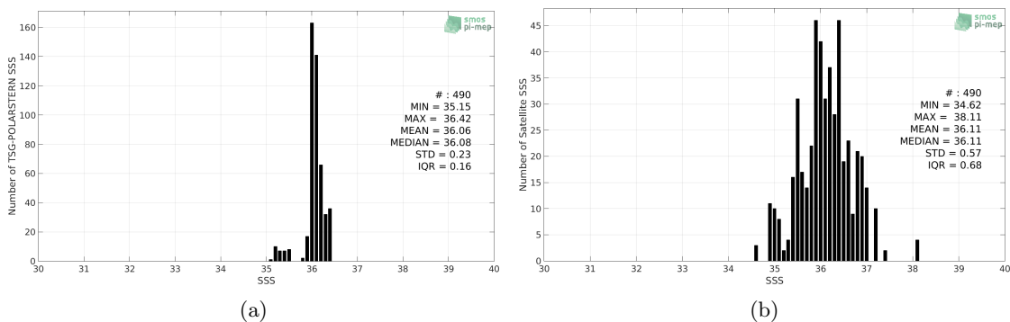
Figure 2: Histograms of SSS from TSG-POLARSTERN (a) and SMOS-L2-DPGS-v662 (b) considering all match-up pairs per bins of 0.1 over the Amazon and Orinoco river plumes Pi-MEP region and for the full satellite product period.
