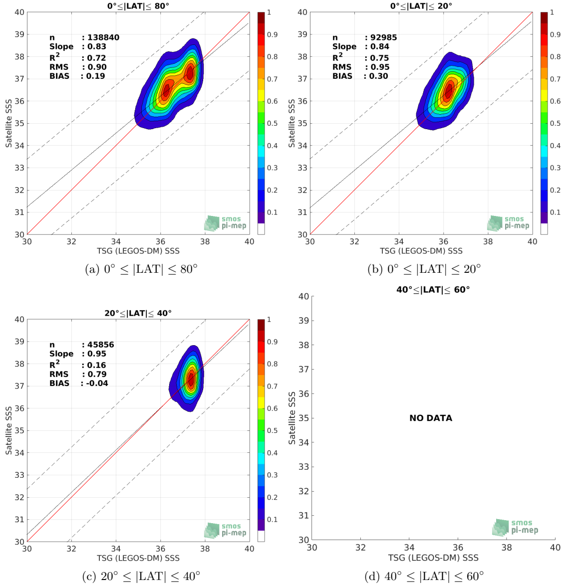
Figure 9: Contour maps of the concentration of SMOS SSS L2 v662 (ESA) SSS (y-axis) versus TSG (LEGOS-DM) SSS (x-axis) at match-up pairs for different latitude bands. For each plot, the red line shows x=y . The black thin and dashed lines indicate a linear fit through the data cloud and the \pm 95\% confidence levels, respectively. The number match-up pairs n , the slope and R^2 coefficient of the linear fit, the root mean square (RMS) and the mean bias between satellite and in situ data are indicated for each latitude band in each plots.
