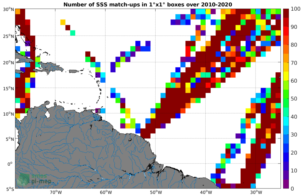
Figure 4: Number of SSS match-ups between TSG (LEGOS-DM) SSS and the SMOS SSS L2 v662 (ESA) SSS product for the Amazon and Orinoco river plumes Pi-MEP region over 1^\circ \times 1^\circ boxes and for the full satellite product period.
