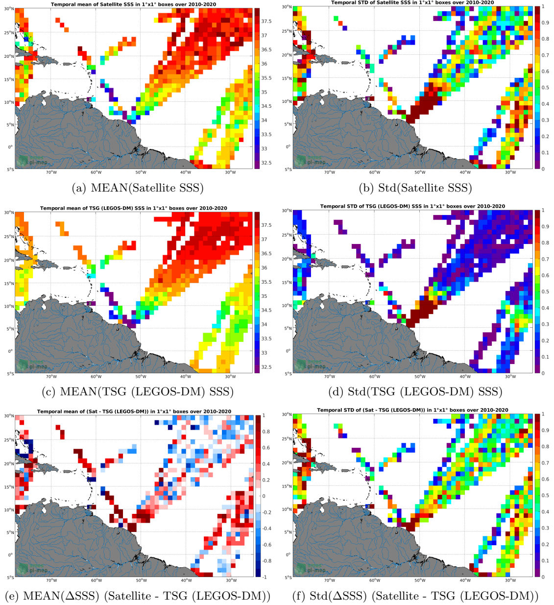
Figure 6: Temporal mean (left) and Std (right) of SSS from SMOS SSS L2 v662 (ESA) (top), TSG (LEGOS-DM) (middle), and of \Delta SSS (Satellite - TSG (LEGOS-DM)). Only match-up pairs are used to generate these maps.
