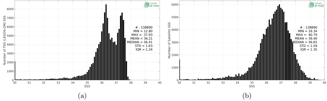
Figure 2: Histograms of SSS from TSG (LEGOS-DM) (a) and SMOS SSS L2 v662 (ESA) (b) considering all match-up pairs per bins of 0.1 over the Amazon and Orinoco river plumes Pi-MEP region and for the full satellite product period.
