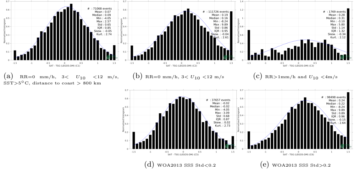
Figure 13: Normalized histogram of \Delta SSS (SMOS SSS L2 v662 (ESA) - TSG (LEGOS-DM)) for 5 different subdatasets corresponding to: RR=0 mm/h, 3 < U_{10} < 12 m/s, SST>5°C, distance to coast > 800 km (a), RR=0 mm/h, 3 < U_{10} < 12 m/s (b), RR>1mm/h and U_{10} < 4 m/s (c), WOA2013 SSS Std<0.2 (d), WOA2013 SSS Std>0.2 (e).
