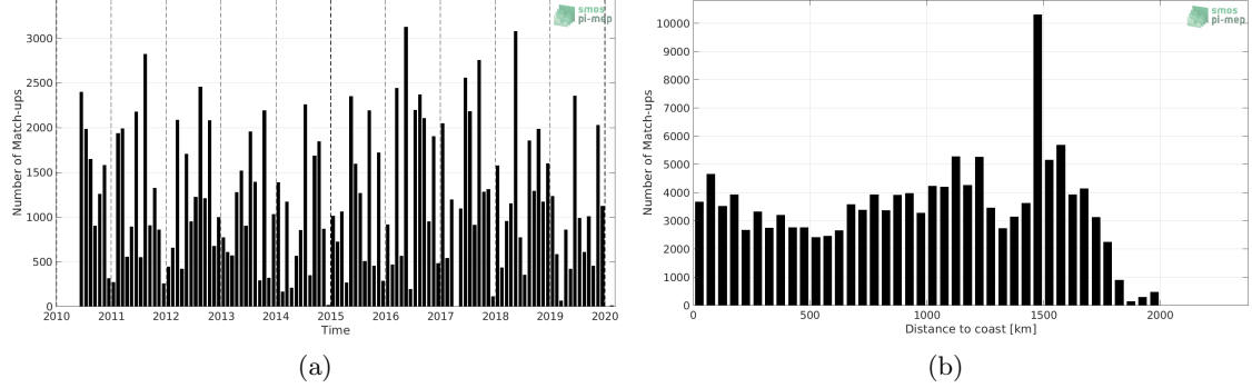
Figure 1: Number of match-ups between TSG (LEGOS-DM) and SMOS SSS L2 v662 (ESA) SSS as a function of time (a) and as function of the distance to coast (b) over the Amazon and Orinoco river plumes Pi-MEP region and for the full satellite product period.
