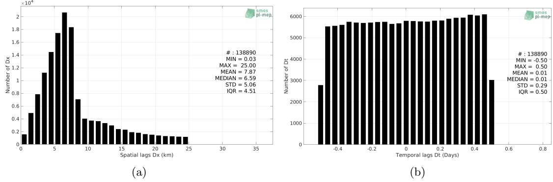
Figure 5: Histograms of the spatial (a) and temporal (b) lags between the location/time of the TSG (LEGOS-DM) measurement and the date of the corresponding SMOS SSS L2 v662 (ESA) SSS pixel.
