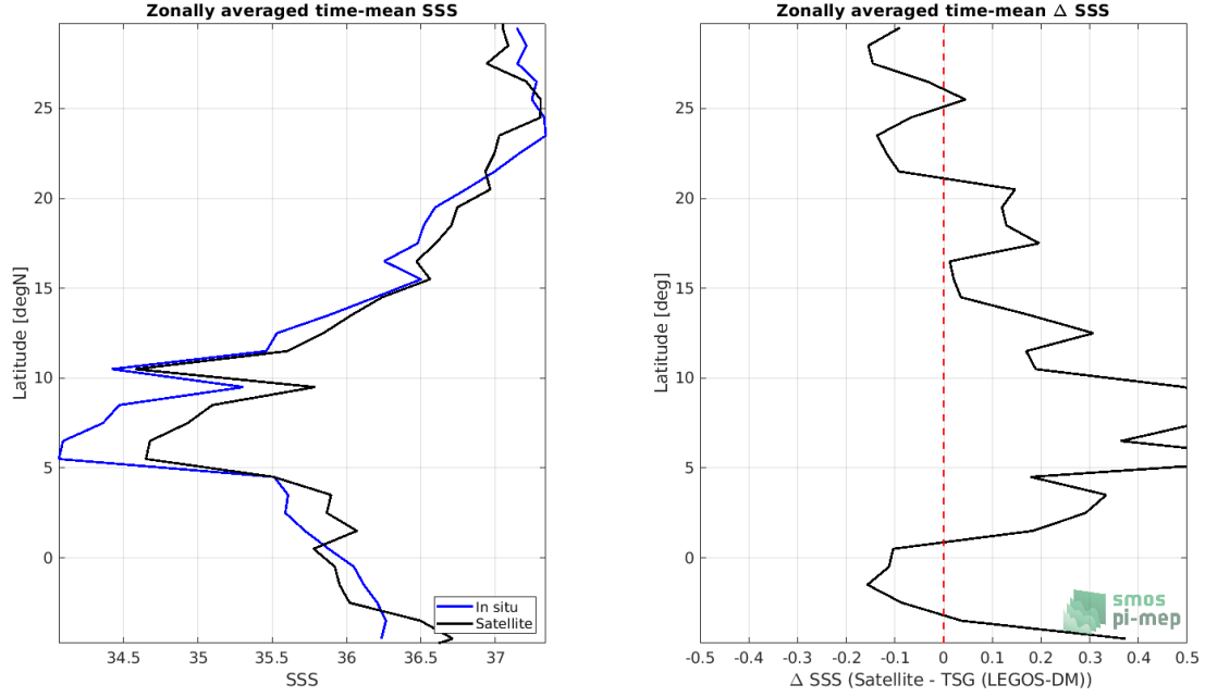
Figure 8: Left panel: Zonal mean SSS from SMOS SSS L2 v662 (ESA) satellite product (black) and from TSG (LEGOS-DM) (blue). Right panel: Zonal mean of \Delta SSS (Satellite - TSG (LEGOS-DM)) for all the collected Pi-MEP match-up pairs estimated over the full satellite product period.
