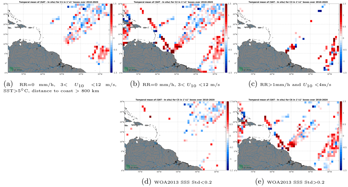
Figure 12: Temporal mean gridded over spatial boxes of size 1^\circ \times 1^\circ of \Delta SSS (SMOS SSS L2 v662 (ESA) - TSG (LEGOS-DM)) for 5 different subdatasets corresponding to: RR=0 mm/h, 3 < U_{10} < 12 m/s, SST > 5^\circ\text{C} , distance to coast > 800 km (a), RR=0 mm/h, 3 < U_{10} < 12 m/s (b), RR > 1 mm/h and U_{10} < 4 m/s (c), WOA2013 SSS Std < 0.2 (d), WOA2013 SSS Std > 0.2 (e).
