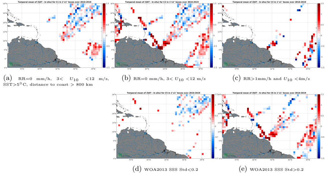
Figure 12: Temporal mean gridded over spatial boxes of size 1^\circ \times 1^\circ of \Delta SSS (SMOS L2 v662 (ESA) - TSG-LEGOS-DM) for 5 different subdatasets corresponding to: RR=0 mm/h, 3 < U_{10} < 12 m/s, SST > 5^\circ C , distance to coast > 800 km (a), RR=0 mm/h, 3 < U_{10} < 12 m/s (b), RR > 1 mm/h and U_{10} < 4 m/s (c), WOA2013 SSS Std < 0.2 (d), WOA2013 SSS Std > 0.2 (e).
