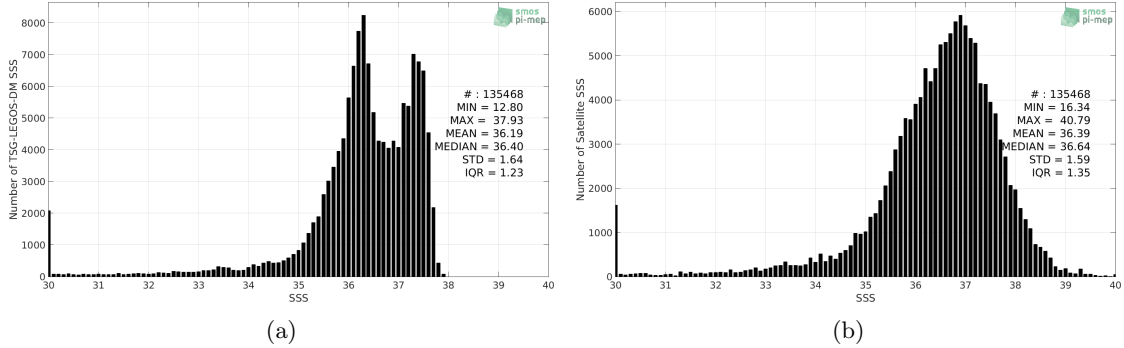
Figure 2: Histograms of SSS from TSG-LEGOS-DM (a) and SMOS L2 v662 (ESA) (b) considering all match-up pairs per bins of 0.1 over the Amazon and Orinoco river plumes Pi-MEP region and for the full satellite product period.
