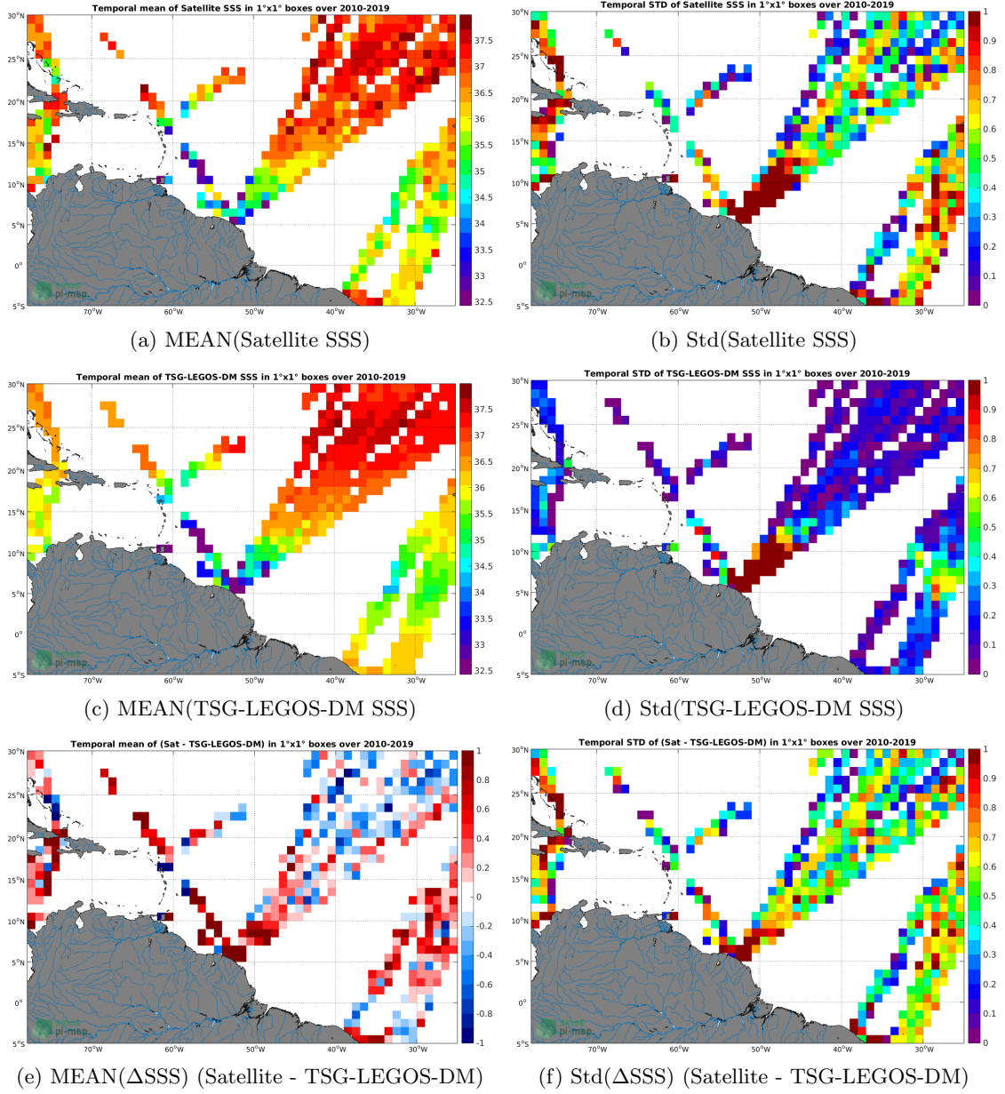
Figure 6: Temporal mean (left) and Std (right) of SSS from SMOS L2 v662 (ESA) (top), TSG-LEGOS-DM (middle), and of \Delta SSS (Satellite - TSG-LEGOS-DM). Only match-up pairs are used to generate these maps.
