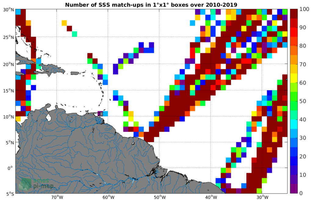
Figure 4: Number of SSS match-ups between TSG-LEGOS-DM SSS and the SMOS L2 v662 (ESA) SSS product for the Amazon and Orinoco river plumes Pi-MEP region over 1^\circ \times 1^\circ boxes and for the full satellite product period.
