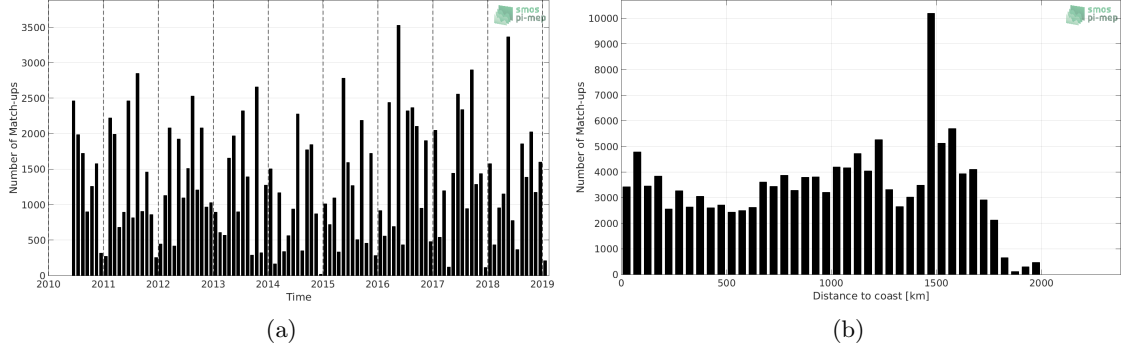
Figure 1: Number of match-ups between TSG-LEGOS-DM and SMOS L2 v662 (ESA) SSS as a function of time (a) and as function of the distance to coast (b) over the Amazon and Orinoco river plumes Pi-MEP region and for the full satellite product period.
