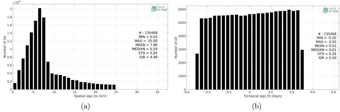
Figure 5: Histograms of the spatial (a) and temporal (b) lags between the time of the TSG-LEGOS-DM measurements and the date of the corresponding SMOS L2 v662 (ESA) SSS product.
