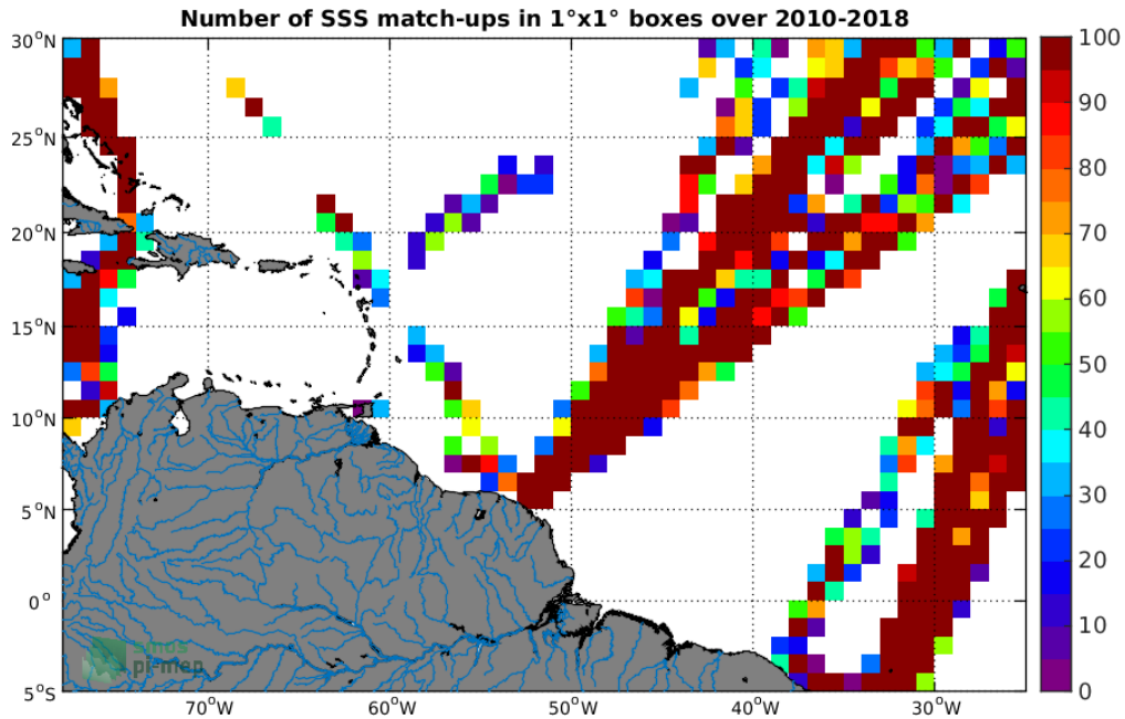
Figure 4: Number of SSS match-ups between TSG-LEGOS-DM SSS and the SMOS-L2-DPGS-v662 SSS product for the Amazon and Orinoco river plumes Pi-MEP region over 1°x1° boxes and for the full satellite product period.
