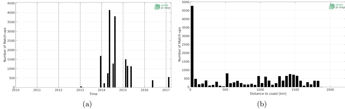
Figure 1: Number of match-ups between TSG (GOSUD-Sailing-ship) and SMOS SSS L2 v662 (ESA) SSS as a function of time (a) and as function of the distance to coast (b) over the Amazon and Orinoco river plumes Pi-MEP region and for the full satellite product period.
