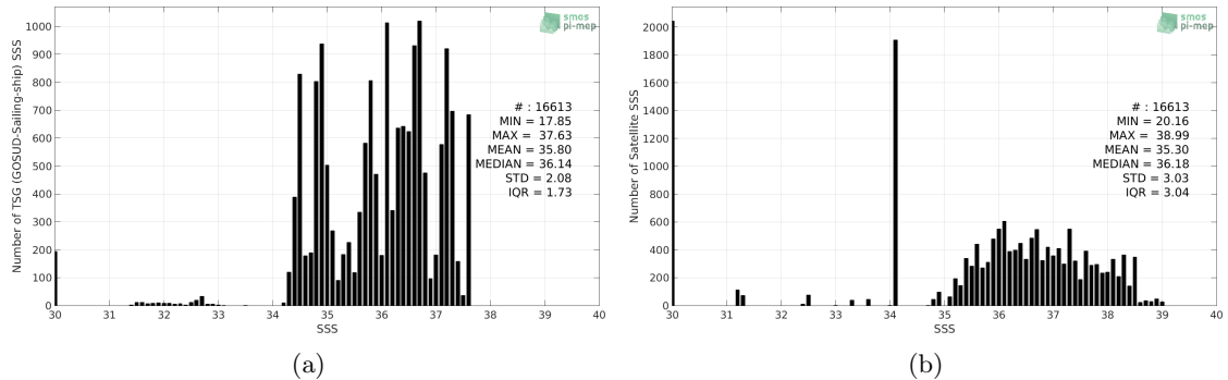
Figure 2: Histograms of SSS from TSG (GOSUD-Sailing-ship) (a) and SMOS SSS L2 v662 (ESA) (b) considering all match-up pairs per bins of 0.1 over the Amazon and Orinoco river plumes Pi-MEP region and for the full satellite product period.
