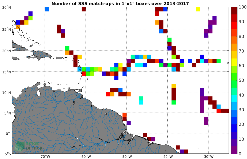
Figure 4: Number of SSS match-ups between TSG (GOSUD-Sailing-ship) SSS and the SMOS SSS L2 v662 (ESA) SSS product for the Amazon and Orinoco river plumes Pi-MEP region over 1^{\circ} \times 1^{\circ} boxes and for the full satellite product period.
