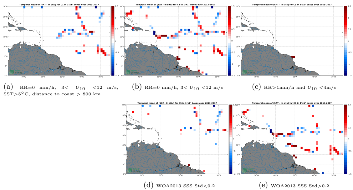
Figure 12: Temporal mean gridded over spatial boxes of size 1°x1° of \Delta SSS (SMOS SSS L2 v662 (ESA) - TSG (GOSUD-Sailing-ship)) for 5 different subdatasets corresponding to:RR=0 mm/h, 3 < U_{10} < 12 m/s, SST > 5°C, distance to coast > 800 km (a), RR=0 mm/h, 3 < U_{10} < 12 m/s (b), RR > 1mm/h and U_{10} < 4m/s (c), WOA2013 SSS Std < 0.2 (d), WOA2013 SSS Std > 0.2 (e).
