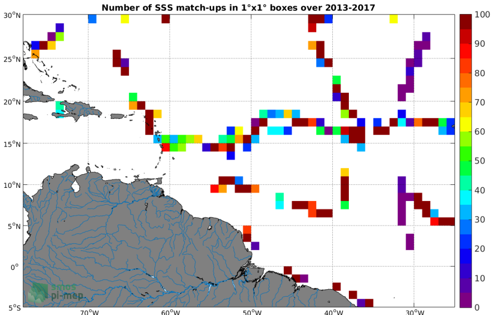
Figure 4: Number of SSS match-ups between TSG (GOSUD-Sailing-ship) SSS and the SMOS SSS L2 v662 (ESA) SSS product for the Amazon and Orinoco river plumes Pi-MEP region over 1°x1° boxes and for the full satellite product period.
