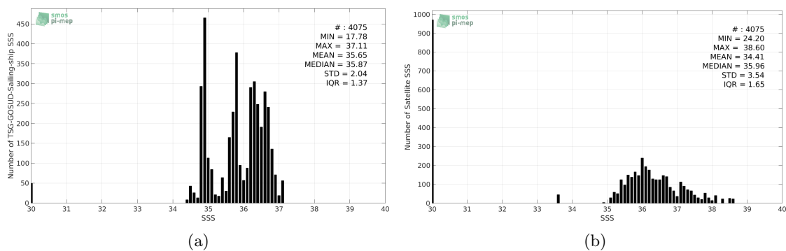
Figure 2: Histograms of SSS from TSG-GOSUD-Sailing-ship (a) and SMOS-L2-DPGS-v662 (b) considering all match-up pairs per bins of 0.1 over the Amazon and Orinoco river plumes Pi-MEP region and for the full satellite product period.
