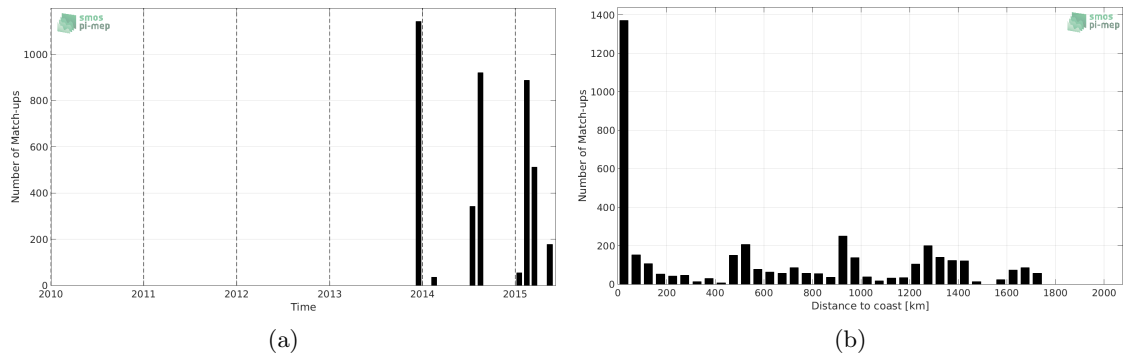
Figure 1: Number of match-ups between TSG-GOSUD-Sailing-ship and SMOS-L2-DPGS-v662 SSS as a function of time (a) and as function of the distance to coast (b) over the Amazon and Orinoco river plumes Pi-MEP region and for the full satellite product period.
